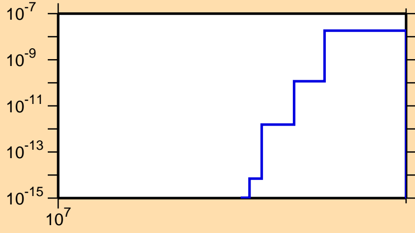
\sigma vs. E for ^{171}\text{Ir}(n,nt)
