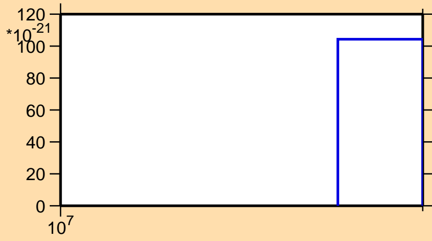
\sigma vs. E for ^{171}\text{Ir}(\text{mt } 42)
