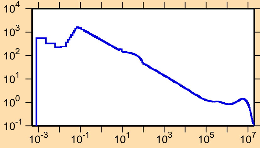
\sigma vs. E for ^{171}\text{Ir}(n,p)
