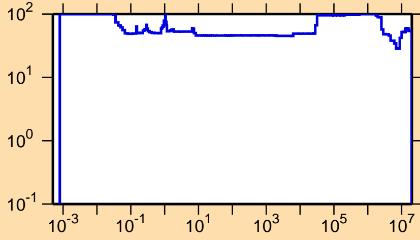
\Delta\sigma/\sigma vs. E for ^{171}\text{Ir}(n,p)
