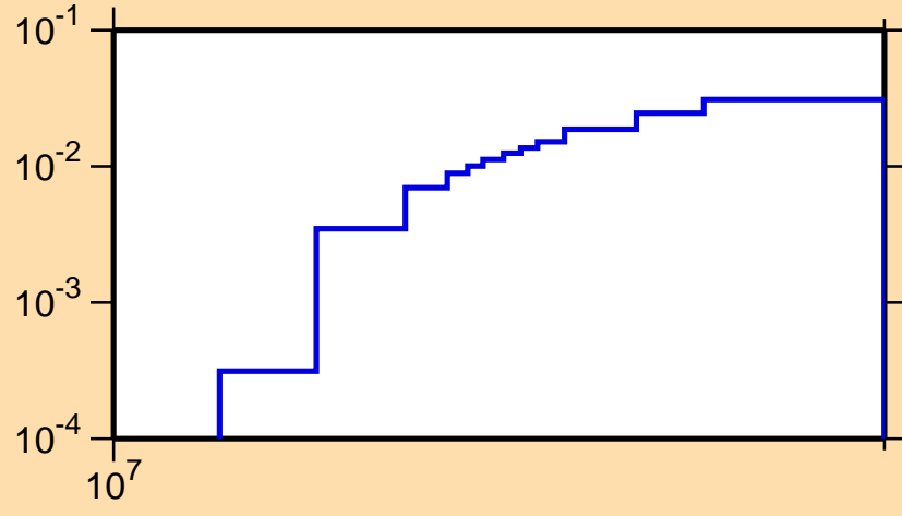
\sigma vs. E for ^{171}\text{Ir}(n,2n)
