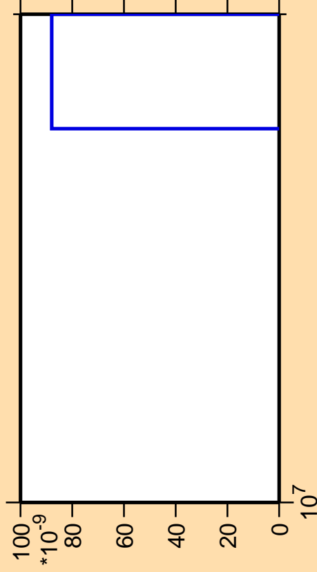
\Delta\sigma/\sigma vs. E for ^{171}\text{Ir}(\text{mt } 42)
