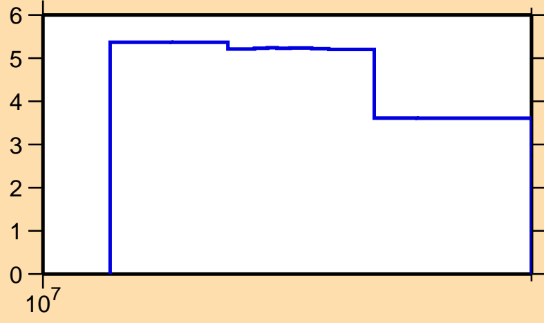
\Delta\sigma/\sigma vs. E for ^{171}\text{Ir}(n,\text{nonel.})
