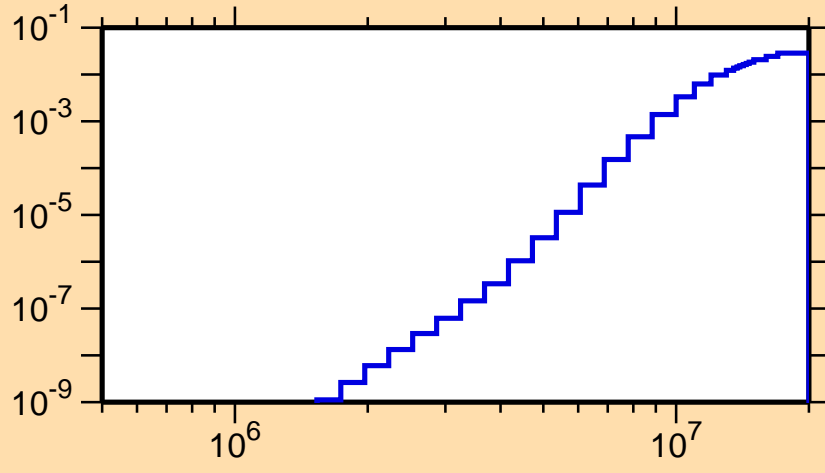
\sigma vs. E for ^{171}\text{Ir}(n,d)
