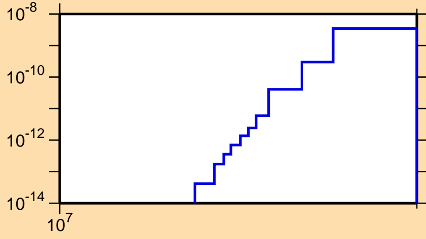
\sigma vs. E for ^{171}\text{Ir}(\text{mt } 34)
