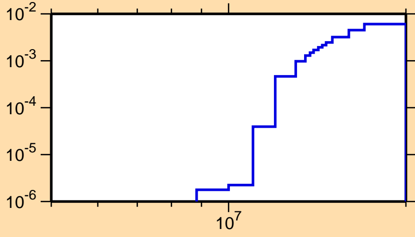
\sigma vs. E for ^{171}\text{Ir}(n,2n\alpha)
