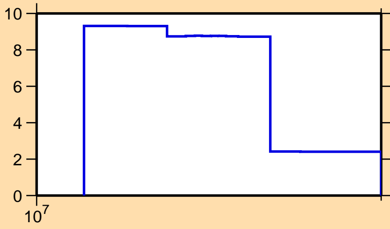
\Delta\sigma/\sigma vs. E for ^{171}\text{Ir}(n,\text{el.})
