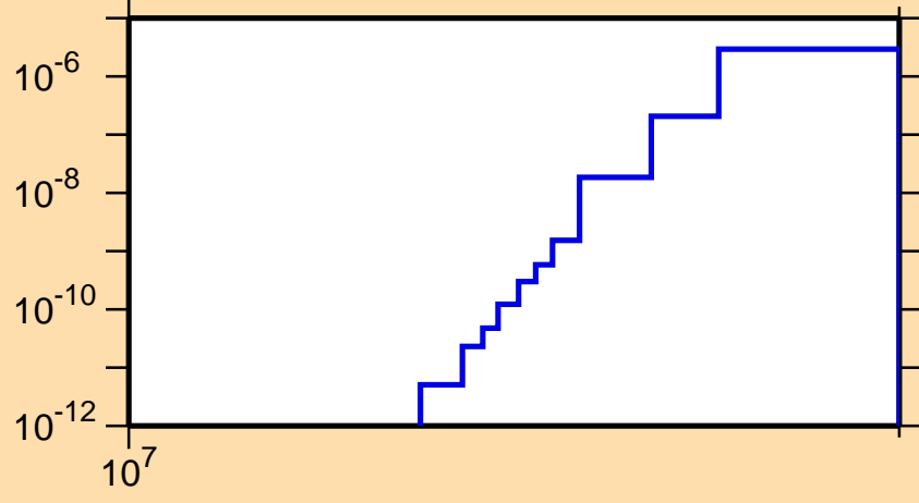
\sigma vs. E for ^{171}\text{Ir}(n,\text{pt})
