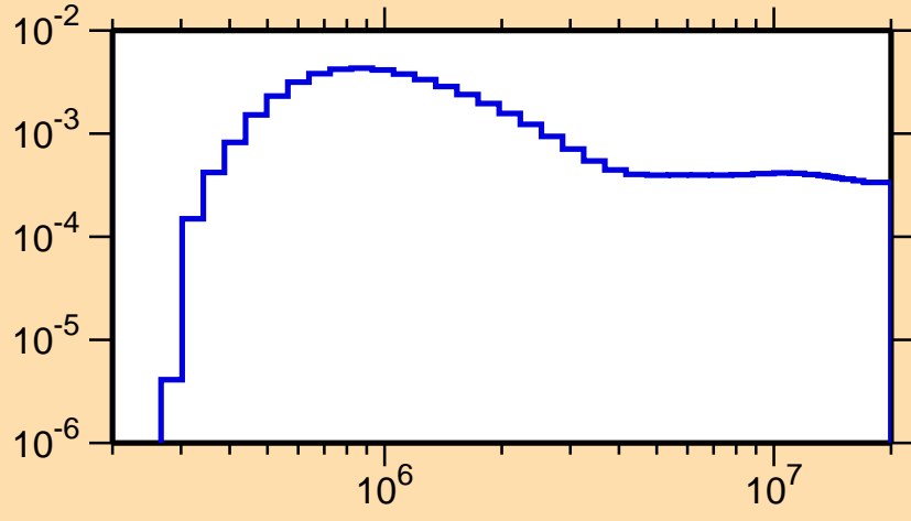
\sigma vs. E for ^{171}\text{Ir}(n,n_3)
