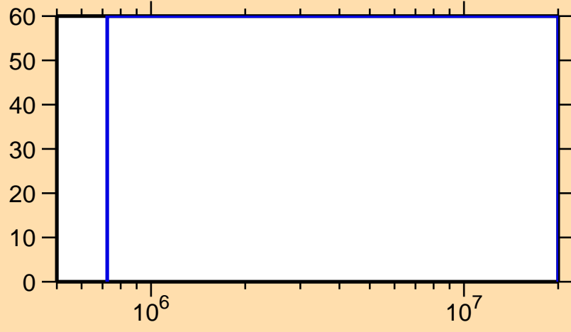
\Delta\sigma/\sigma vs. E for ^{171}\text{Ir}(n,n\text{cont.})
