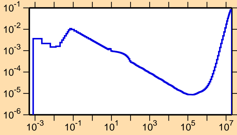
\sigma vs. E for ^{171}\text{Ir}(n,p\alpha)
