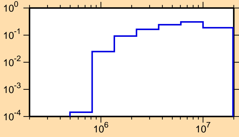
\sigma vs. E for ^{171}\text{Ir}(n,n\text{cont.})
