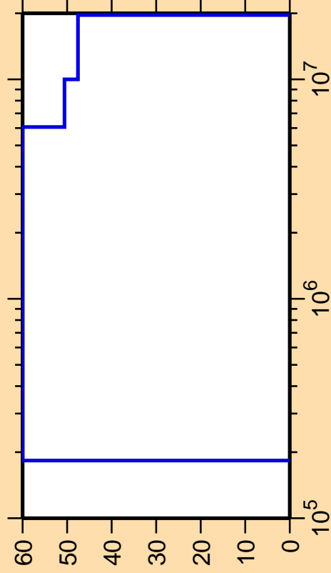
\Delta\sigma/\sigma vs. E for ^{171}\text{Ir}(n,\text{inel.})
