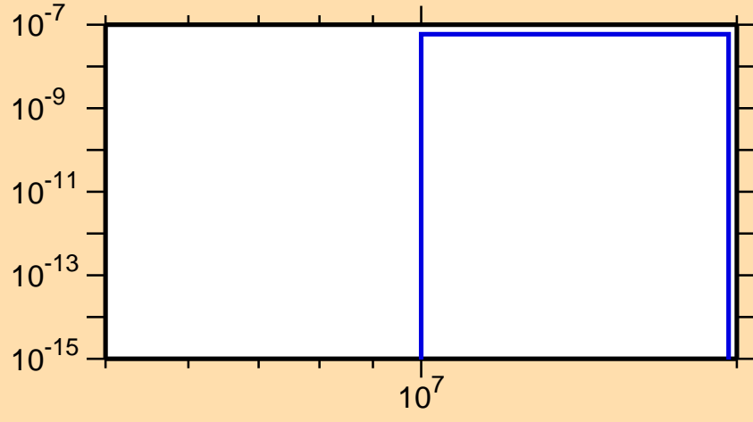
\sigma vs. E for ^{171}\text{Ir}(n,nd)
