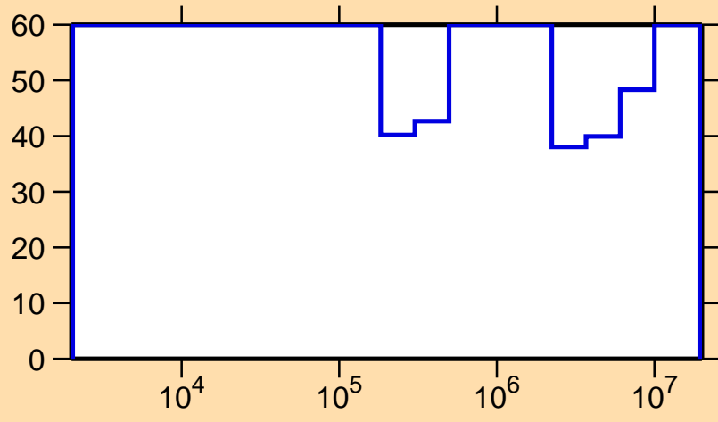
\Delta\sigma/\sigma vs. E for ^{171}\text{Ir}(n,ncont.)
