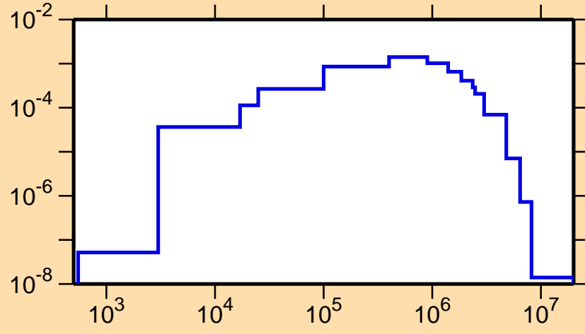
\sigma vs. E for ^{171}\text{Ir}(n,n_2)
