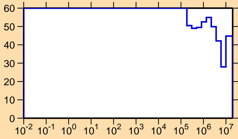
\Delta\sigma/\sigma vs. E for ^{172}\text{Ir}(n,p)
