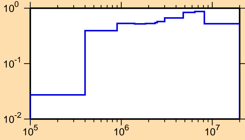
\sigma vs. E for ^{172}\text{Ir}(n,\text{inel.})
