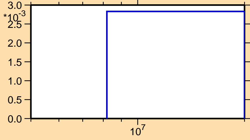
\sigma vs. E for ^{172}\text{Ir}(n,2np)
