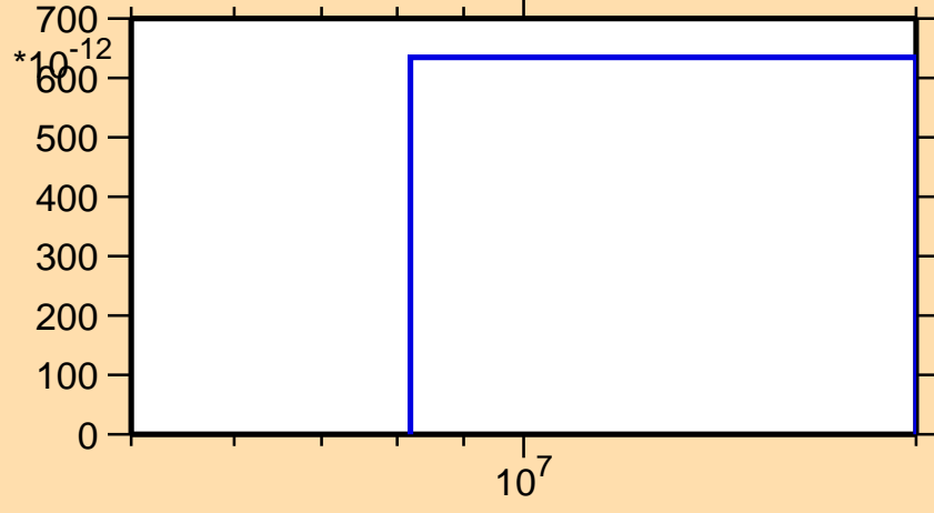
\sigma vs. E for ^{172}\text{Ir}(\text{mt } 34)
