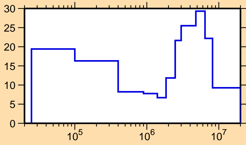
\Delta\sigma/\sigma vs. E for ^{172}\text{Ir}(n,\text{el.})
