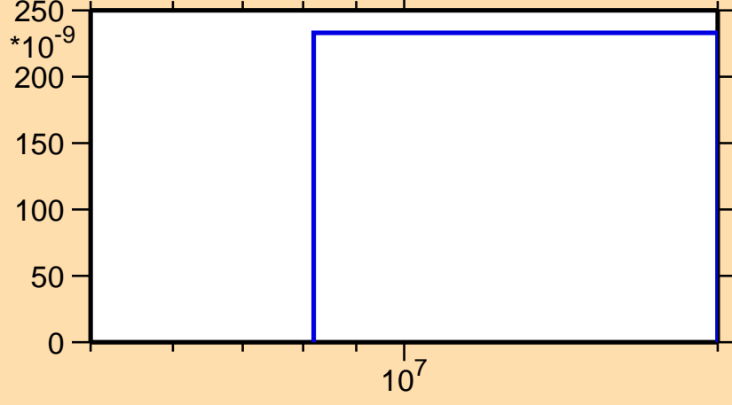
\sigma vs. E for ^{172}\text{Ir}(n,\text{pt})
