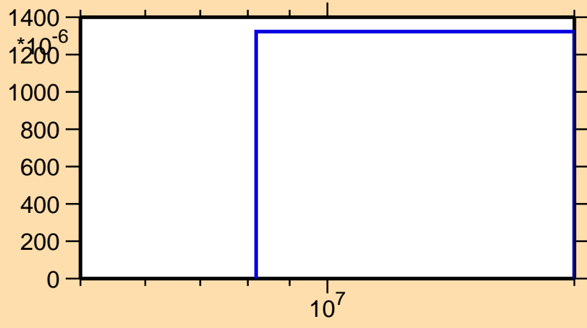
\sigma vs. E for ^{172}\text{Ir}(n,2n\alpha)
