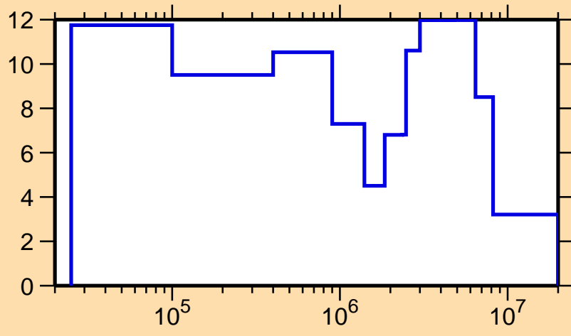
\Delta\sigma/\sigma vs. E for ^{172}\text{Ir}(n,\text{tot.})
