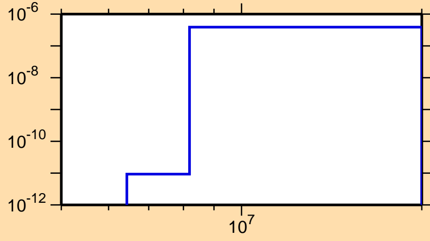
\sigma vs. E for ^{172}\text{Ir}(\text{mt117})
