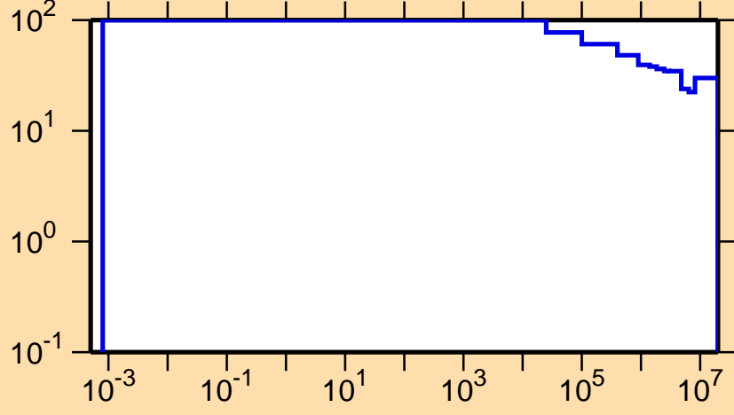
\Delta\sigma/\sigma vs. E for ^{172}\text{Ir}(n,p)
