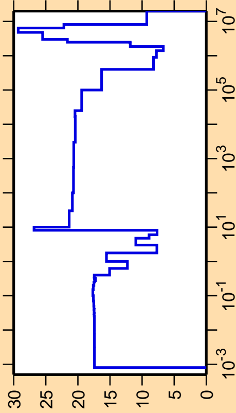
\Delta\sigma/\sigma vs. E for ^{172}\text{Ir}(n,\text{el.})
