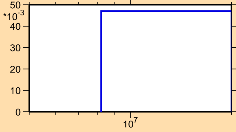
\sigma vs. E for ^{172}\text{Ir}(n,2n)
