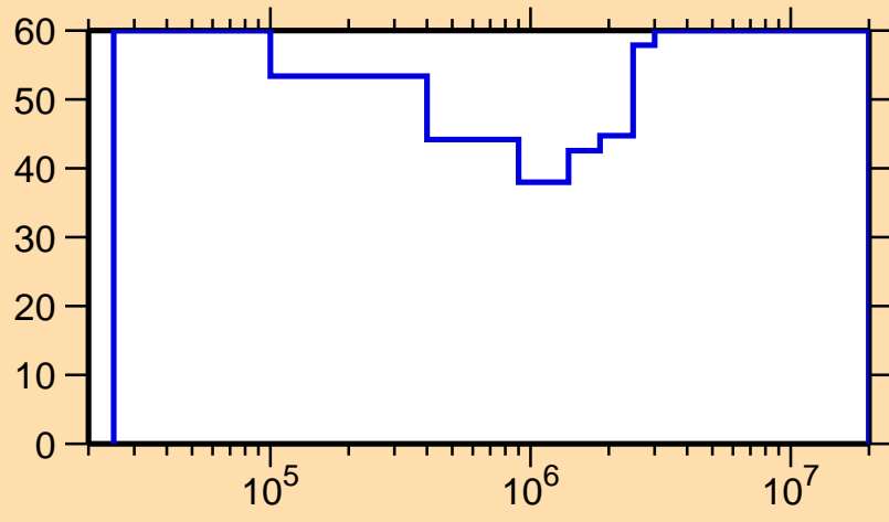
\Delta\sigma/\sigma vs. E for ^{172}\text{Ir}(n,n_1)
