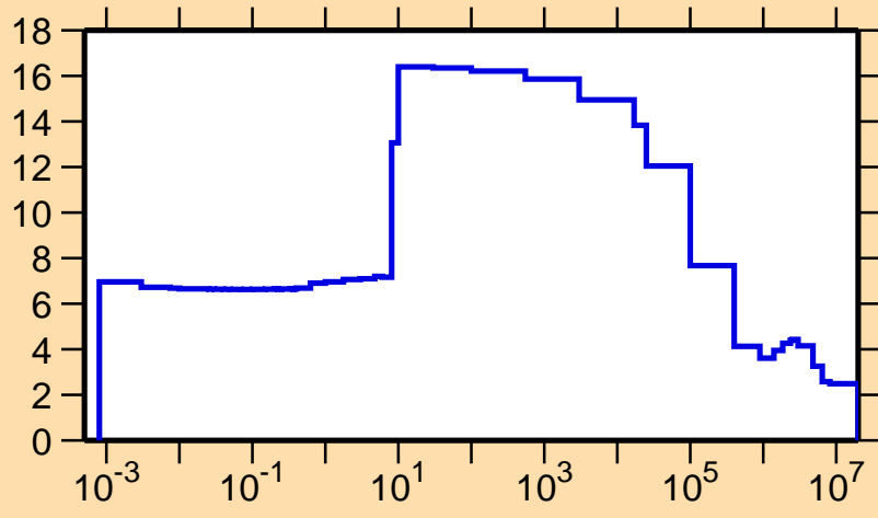
\sigma vs. E for ^{172}\text{Ir}(n,\text{el.})
