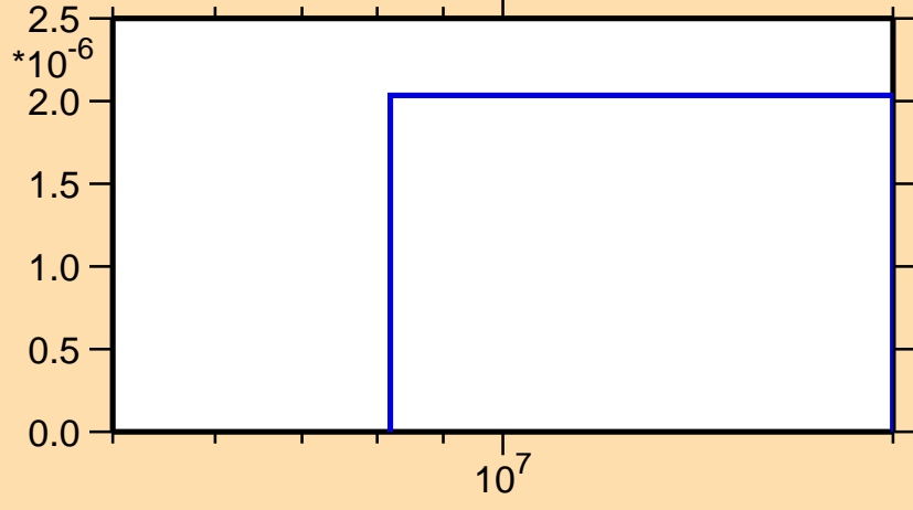
\sigma vs. E for ^{172}\text{Ir}(n,\text{nd})
