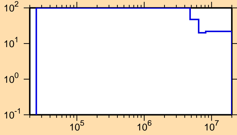
\Delta\sigma/\sigma vs. E for ^{172}\text{Ir}(n,n\text{cont.})
