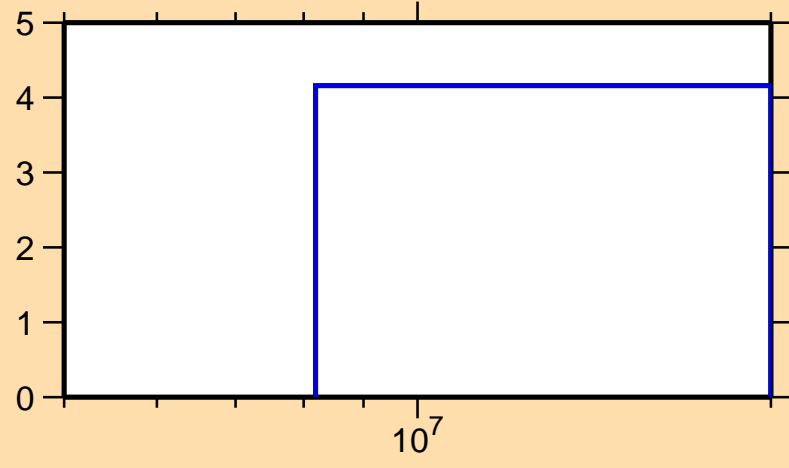
\Delta\sigma/\sigma vs. E for ^{172}\text{Ir}(n,\text{nonel.})
