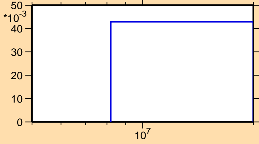
\sigma vs. E for ^{173}\text{Ir}(n,2n)
