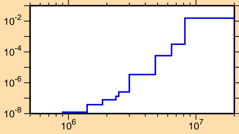
\sigma vs. E for ^{173}\text{Ir}(n,n\alpha)
