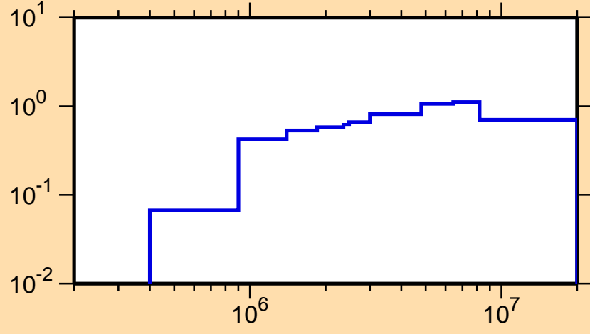
\sigma vs. E for ^{173}\text{Ir}(n,\text{inel.})
