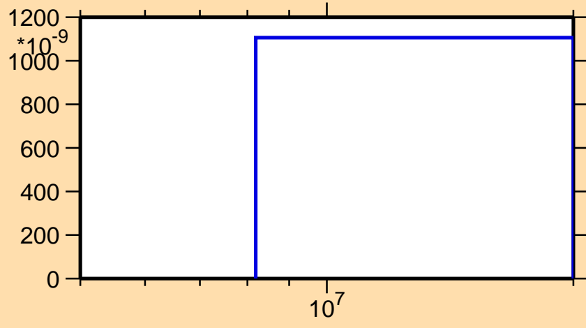
\sigma vs. E for ^{173}\text{Ir}(n,2n\alpha)
