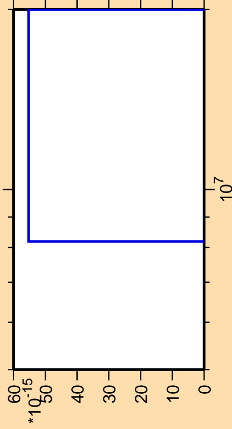
\Delta\sigma/\sigma vs. E for ^{173}\text{Ir}(\text{mt } 42)
