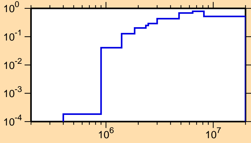
\sigma vs. E for ^{173}\text{Ir}(n,n\text{cont.})
