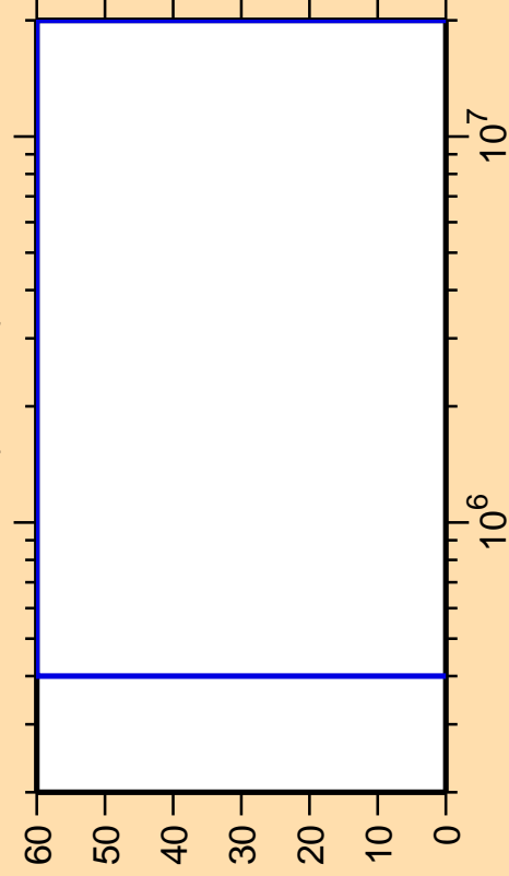
\Delta\sigma/\sigma vs. E for ^{173}\text{Ir}(n,\text{inel.})
