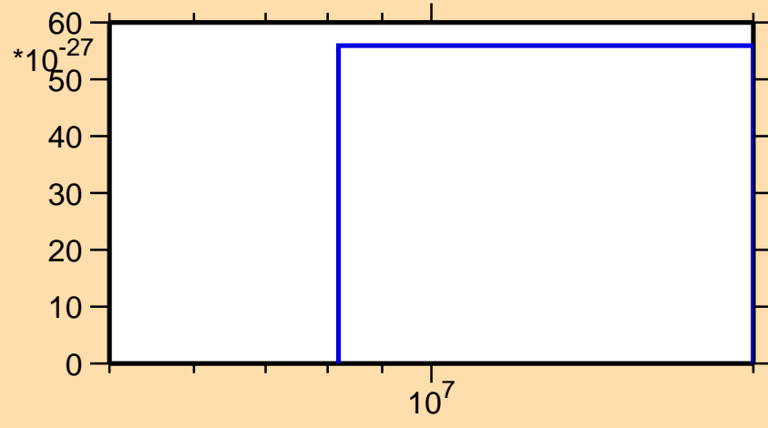
\sigma vs. E for ^{173}\text{Ir}(\text{mt } 42)
