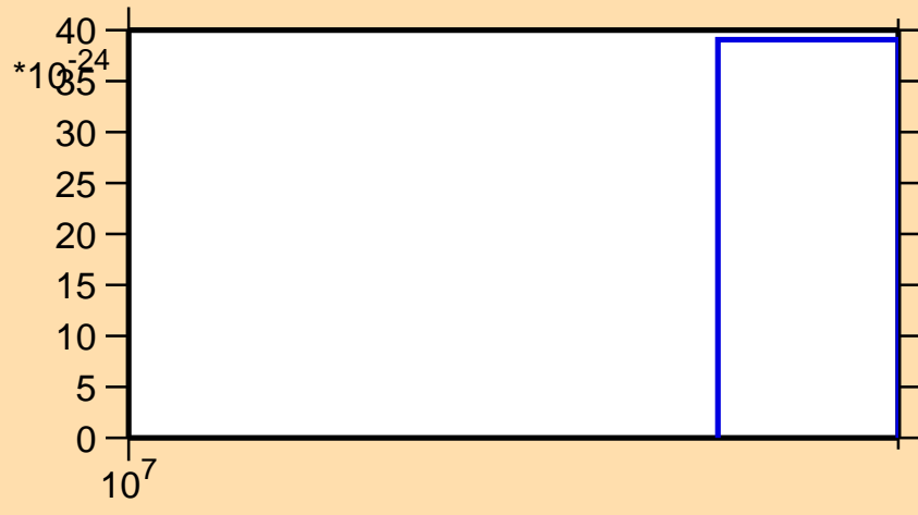
\sigma vs. E for ^{173}\text{Ir}(\text{mt } 42)
