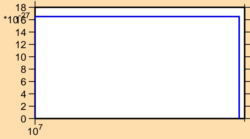
\sigma vs. E for ^{173}\text{Ir} (mt 42)
