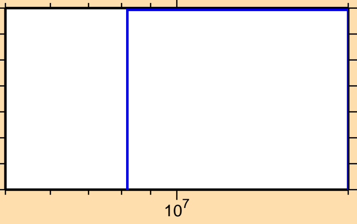
\sigma vs. E for ^{173}\text{Ir}(n,\text{nd})
