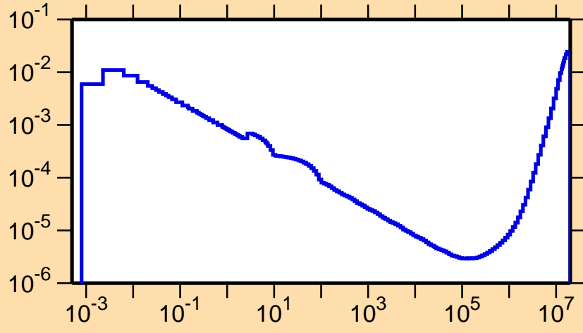
\sigma vs. E for ^{174}\text{Ir}(n,p\alpha)
