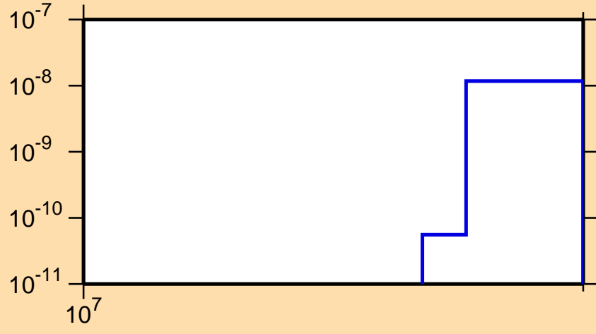
\sigma vs. E for ^{174}\text{Ir}(n,nt)
