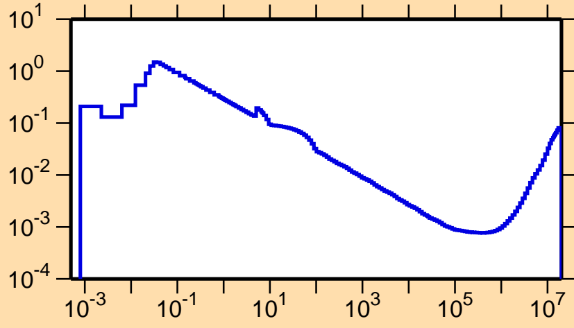
\sigma vs. E for ^{177}\text{Ir}(n,\alpha)
