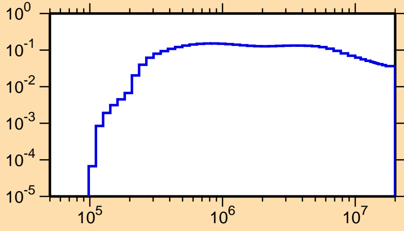
\sigma vs. E for ^{177}\text{Ir}(n,n_4)
