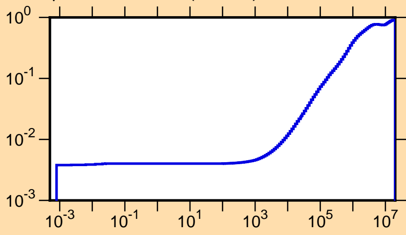
\mu vs. E for ^{178}\text{Ir}(\text{mt251})
