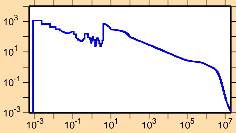
\sigma vs. E for ^{178}\text{Ir}(n,\gamma)
