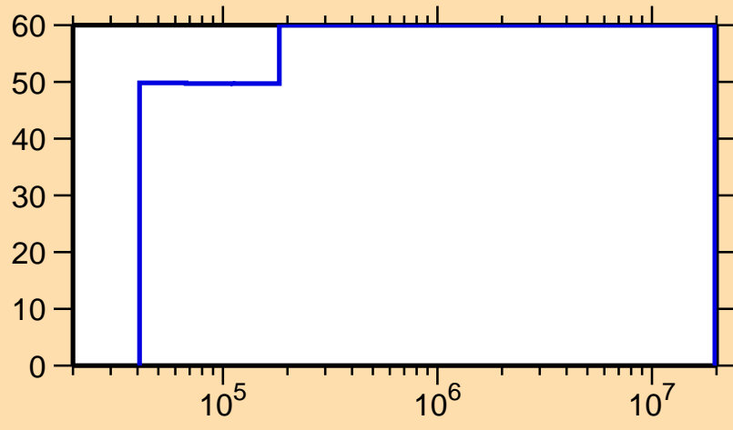
\Delta\sigma/\sigma vs. E for ^{178}\text{Ir}(n,n_1)
