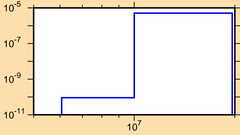
\sigma vs. E for ^{178}\text{Ir}(n,\text{He3})
