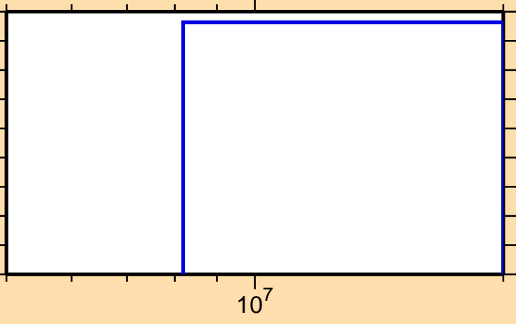
\sigma vs. E for ^{178}\text{Ir}(n,nt)
