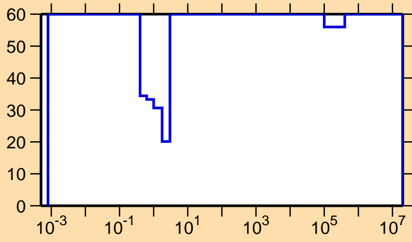
\Delta\sigma/\sigma vs. E for ^{178}\text{Ir}(n,\gamma)
