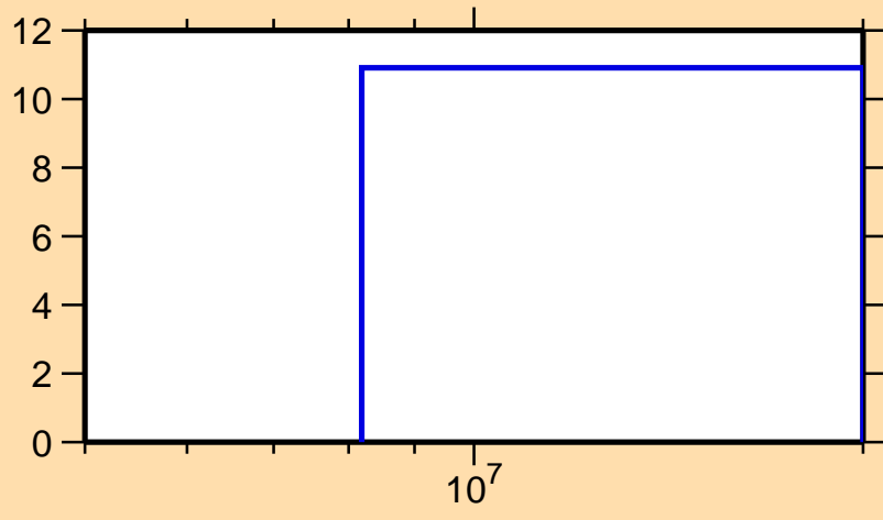
\Delta\sigma/\sigma vs. E for ^{178}\text{Ir}(n,\text{tot.})
