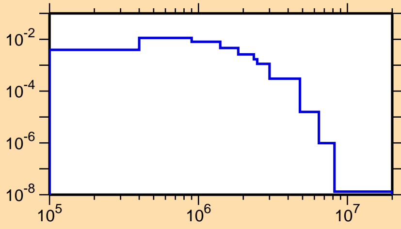
\sigma vs. E for ^{178}\text{Ir}(n,n_2)
