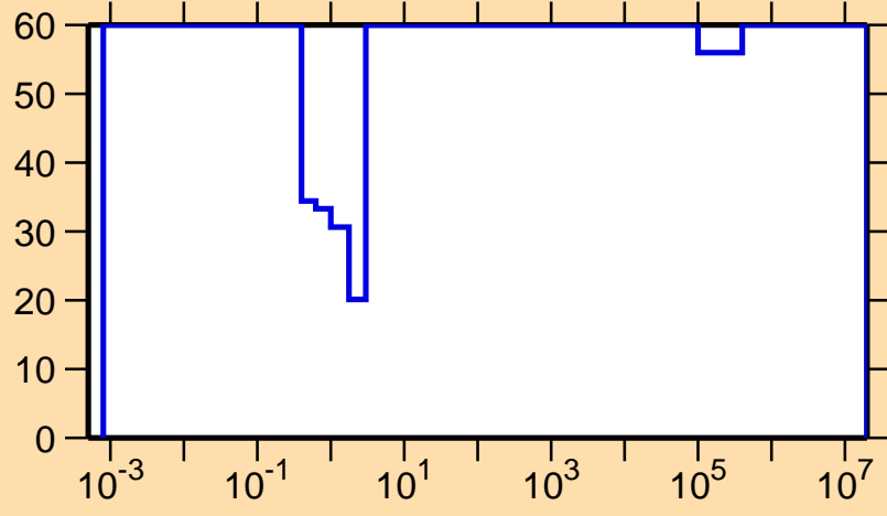
\Delta\sigma/\sigma vs. E for ^{178}\text{Ir}(n,\gamma)
