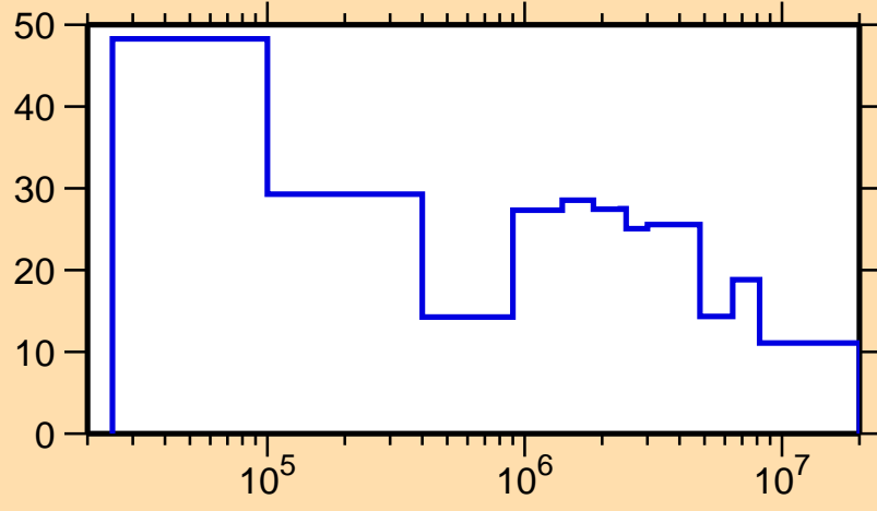
\Delta\sigma/\sigma vs. E for ^{178}\text{Ir}(n,\text{el.})
