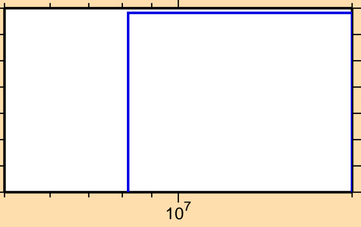
\sigma vs. E for ^{178}\text{Ir}(n,\text{pt})
