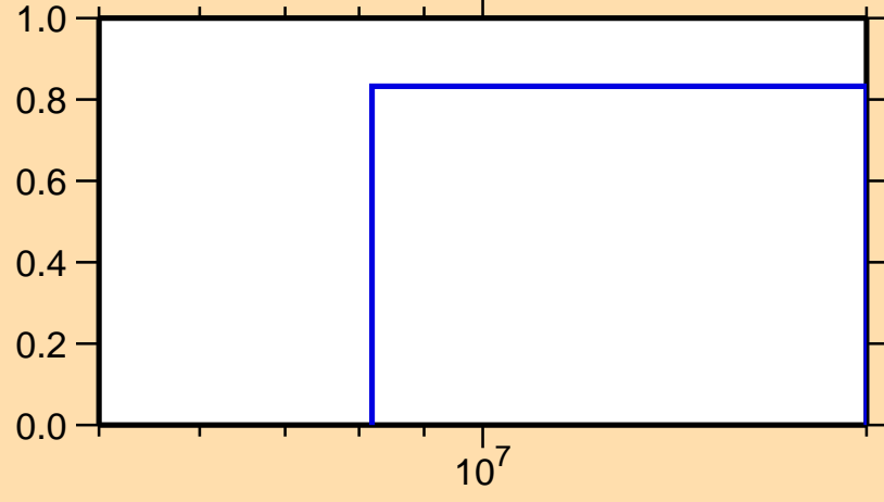
\sigma vs. E for ^{178}\text{Ir}(n,2n)
