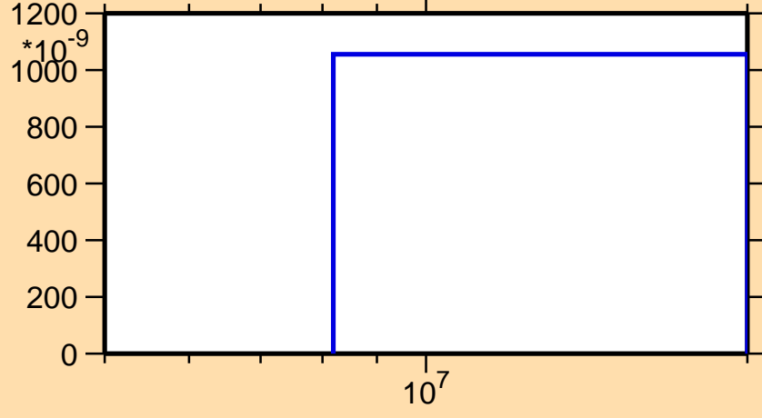
\sigma vs. E for ^{178}\text{Ir}(n,3n)
