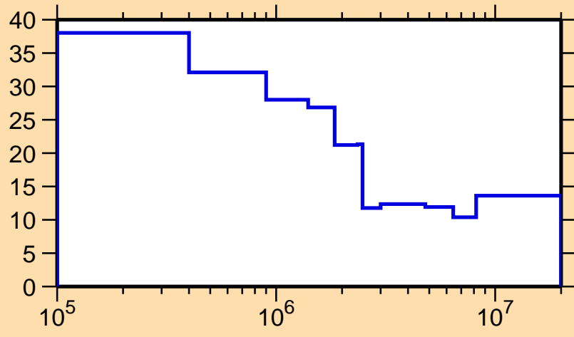
\Delta\sigma/\sigma vs. E for ^{178}\text{Ir}(n,\text{nonel.})
