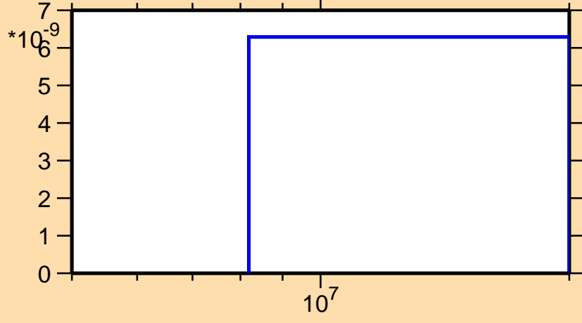
\sigma vs. E for ^{178}\text{Ir}(n,\text{pd})
