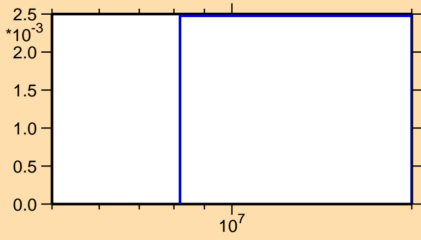
\sigma vs. E for ^{178}\text{Ir}(n,2np)
