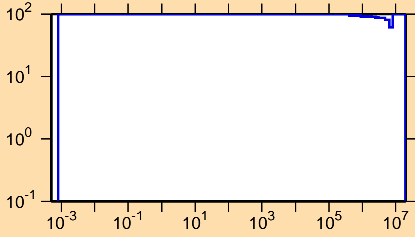
\Delta\sigma/\sigma vs. E for ^{178}\text{Ir}(n,p)
