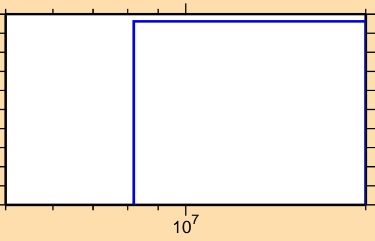
\sigma vs. E for ^{178}\text{Ir}(n,2n\alpha)
