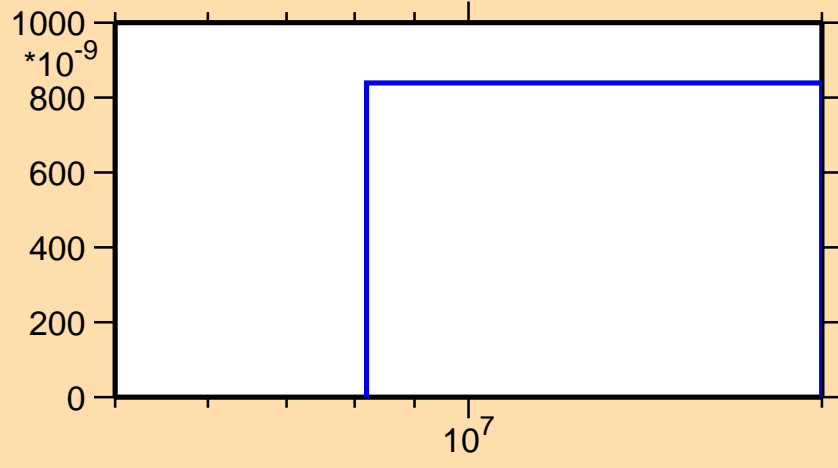
\sigma vs. E for ^{178}\text{Ir}(\text{mt } 45)
