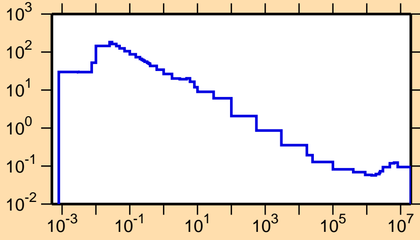
\sigma vs. E for ^{178}\text{Ir}(n,p)
