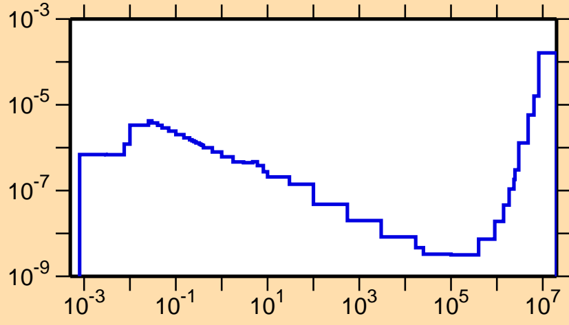
\sigma vs. E for ^{178}\text{Ir}(n,p\alpha)
