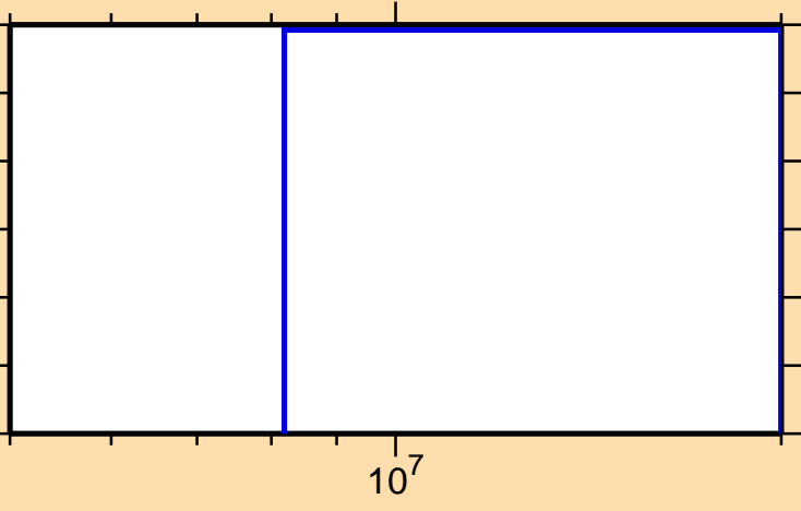
\sigma vs. E for ^{178}\text{Ir}(\text{mt } 42)
