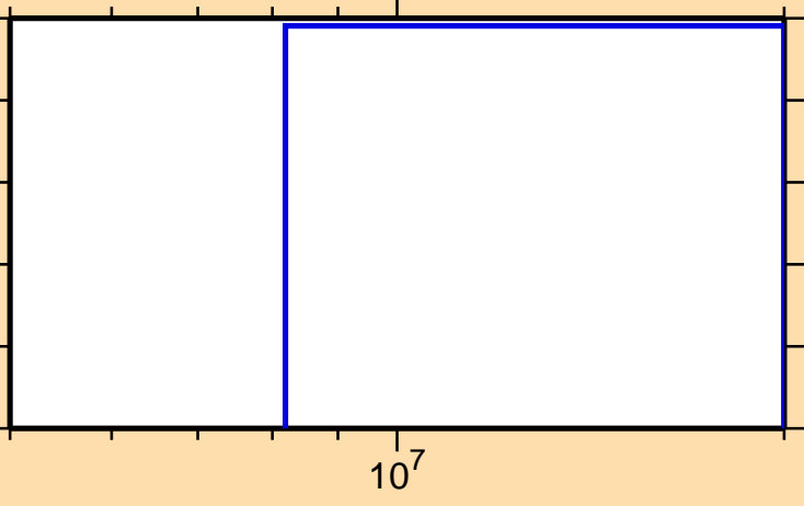
\sigma vs. E for ^{178}\text{Ir}(\text{mt117})
