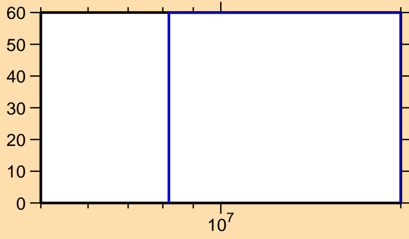
\Delta\sigma/\sigma vs. E for ^{178}\text{Ir}(n,\text{inel.})
