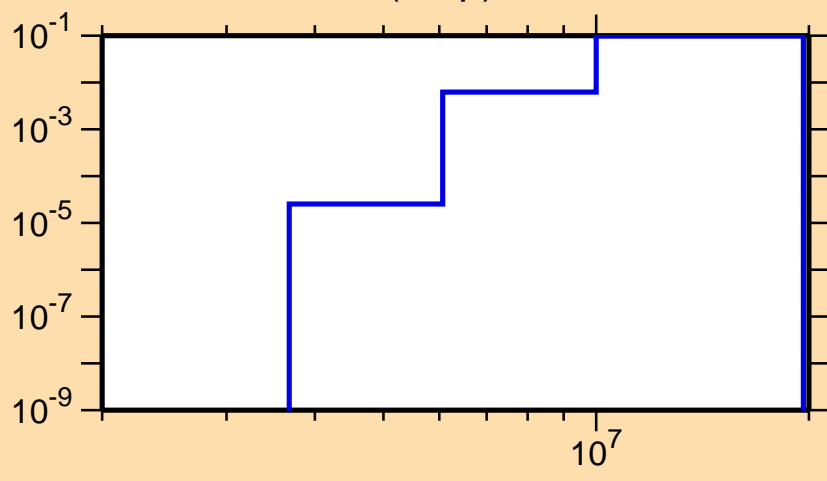
\sigma vs. E for ^{179}\text{Ir}(n,np)
