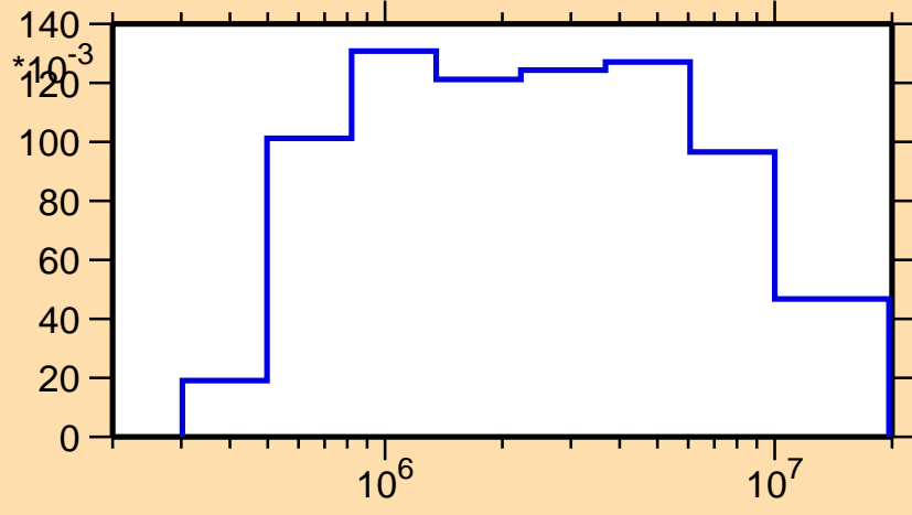
\sigma vs. E for ^{179}\text{Ir}(n,n_4)
