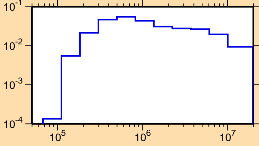
\sigma vs. E for ^{179}\text{Ir}(n,n_1)
