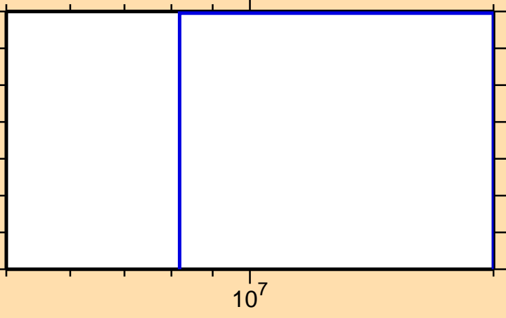
\sigma vs. E for ^{179}\text{Ir}(n,\text{nd})
