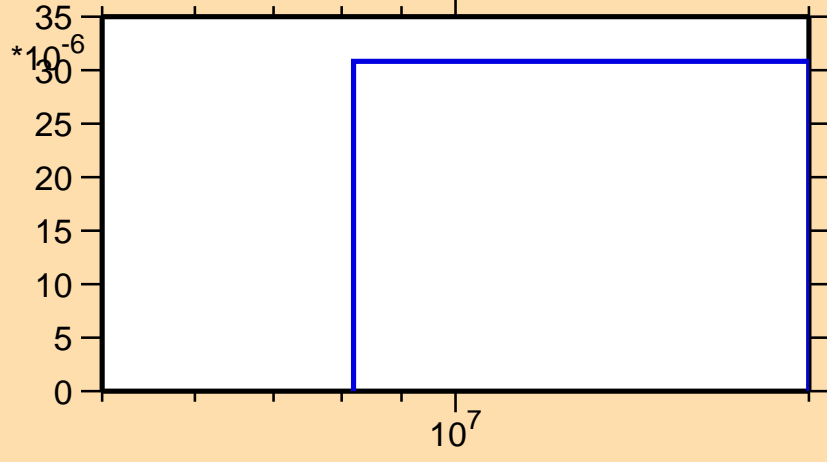
\sigma vs. E for ^{179}\text{Ir}(n,2np)
