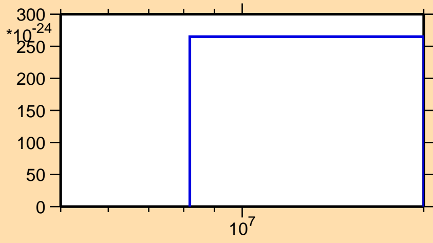
\sigma vs. E for ^{179}\text{Ir}(\text{mt } 42)
