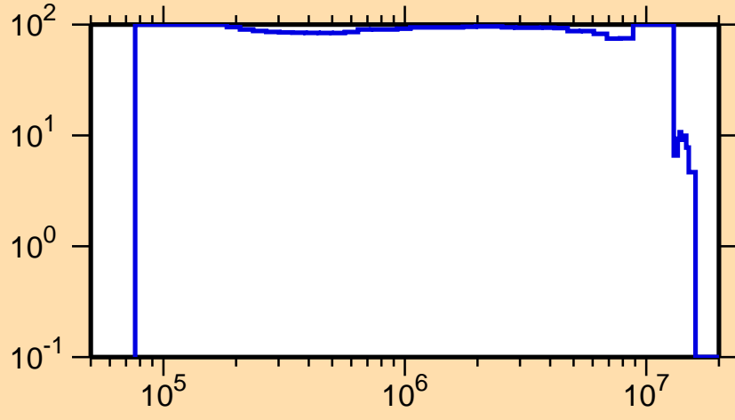
\Delta\sigma/\sigma vs. E for ^{180}\text{Ir}(n,n_1)
