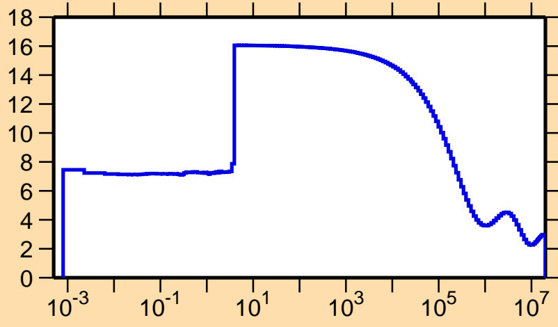
\sigma vs. E for ^{180}\text{Ir}(n,\text{el.})
