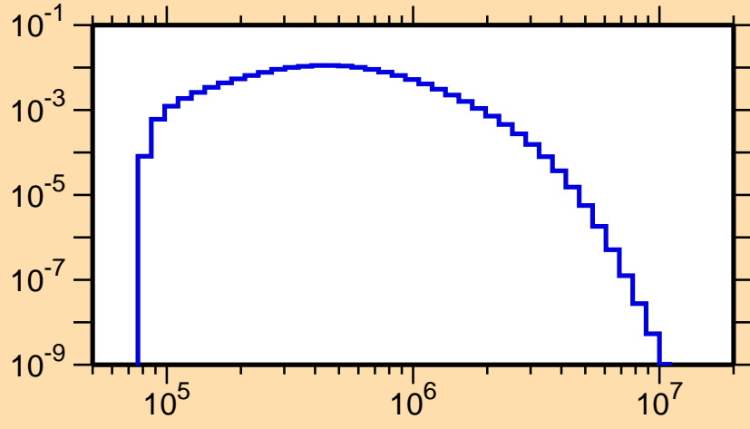
\sigma vs. E for ^{180}\text{Ir}(n,n_1)
