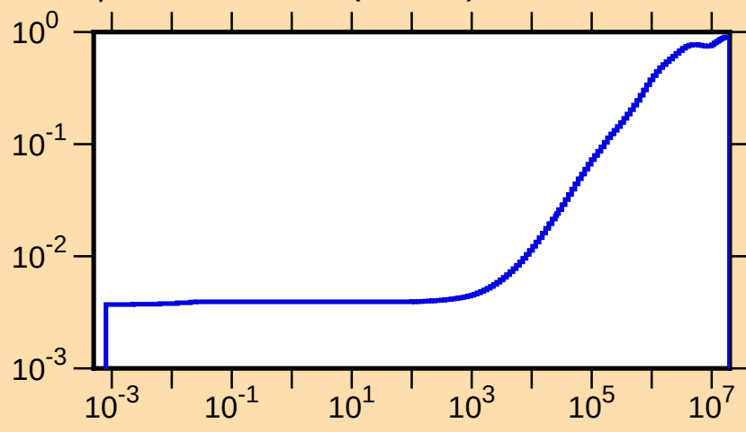
\mu vs. E for ^{182}\text{Ir}(\text{mt251})
