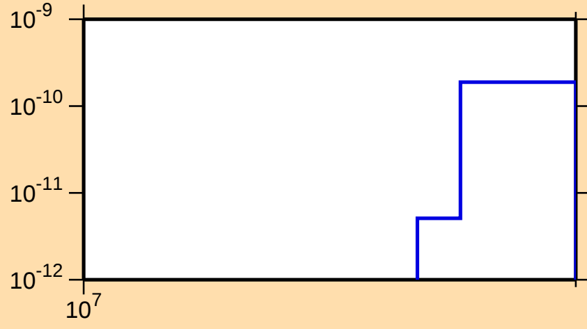
\sigma vs. E for ^{182}\text{Ir}(n,\text{pt})
