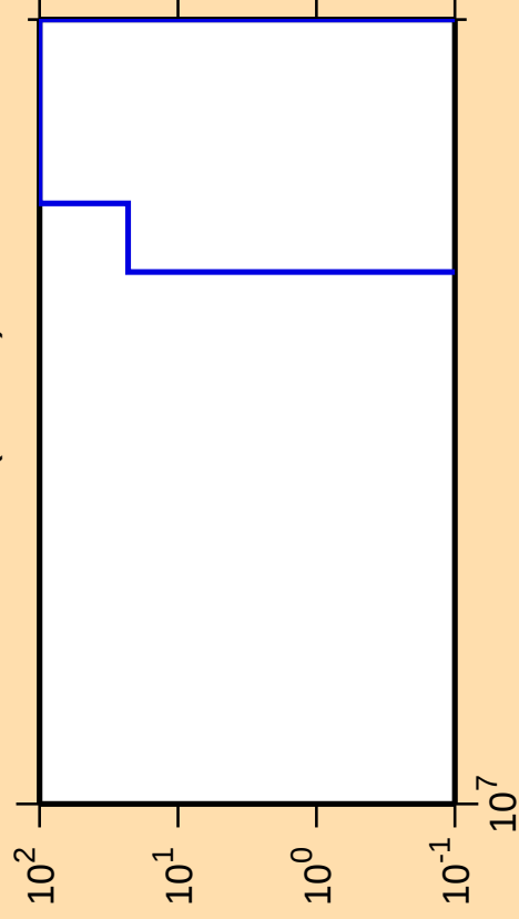
\Delta\sigma/\sigma vs. E for ^{182}\text{Ir}(\text{mt } 34)
