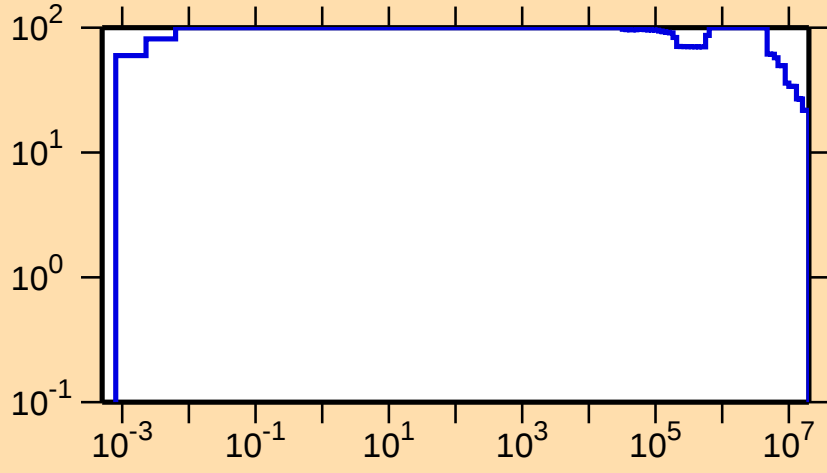
\Delta\sigma/\sigma vs. E for ^{182}\text{Ir}(n,p)
