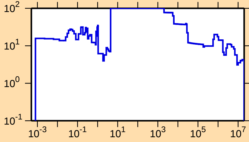
\Delta\sigma/\sigma vs. E for ^{182}\text{Ir}(n,\text{tot.})
