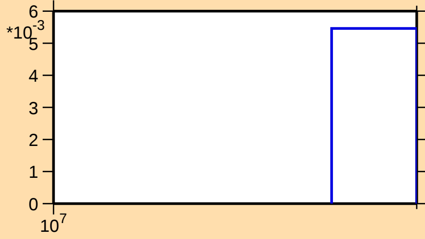
\sigma vs. E for ^{182}\text{Ir}(n,3n)
