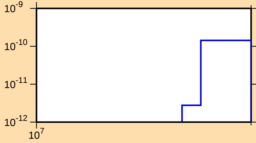
\sigma vs. E for ^{182}\text{Ir}(\text{mt } 34)
