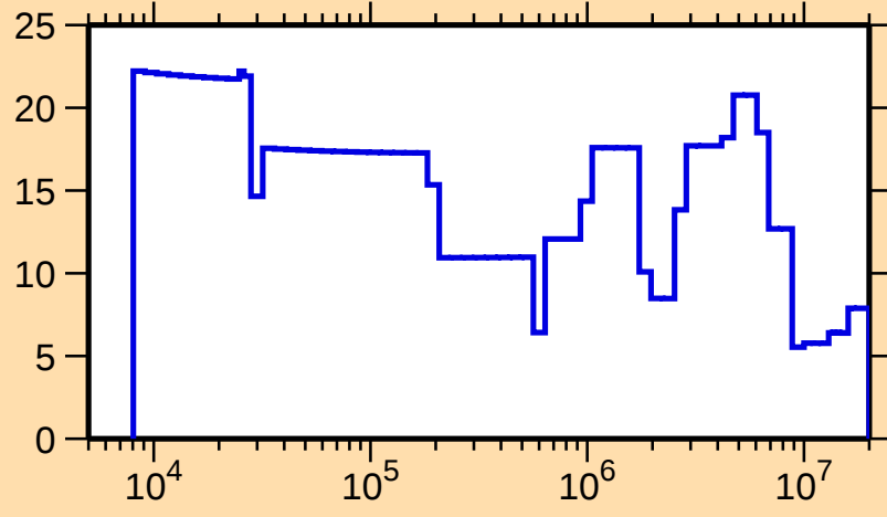
\Delta\sigma/\sigma vs. E for ^{182}\text{Ir}(n,\text{el.})
