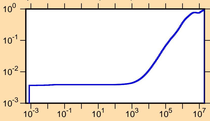
\mu vs. E for ^{183}\text{Ir}(\text{mt251})
