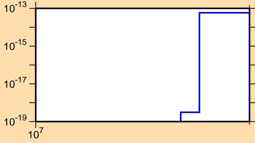
\sigma vs. E for ^{183}\text{Ir}(n,3n\alpha)
