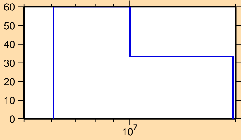
\Delta\sigma/\sigma vs. E for ^{183}\text{Ir}(n,2n)
