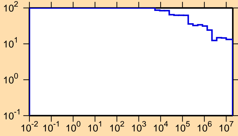
\Delta\sigma/\sigma vs. E for ^{183}\text{Ir}(n,\text{nonel.})
