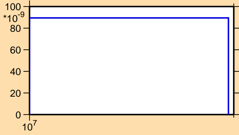
\sigma vs. E for ^{183}\text{Ir}(n,\text{nd})
