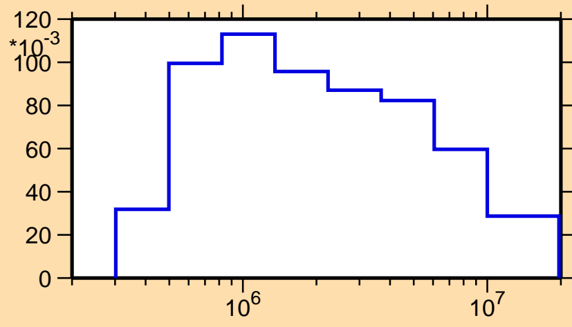
\sigma vs. E for ^{183}\text{Ir}(n,n_4)
