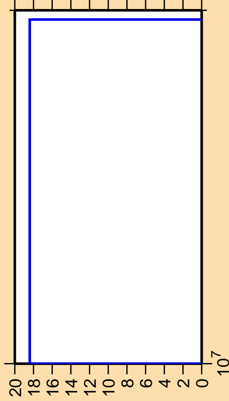
\Delta\sigma/\sigma vs. E for ^{183}\text{Ir}(n,\text{pd})
