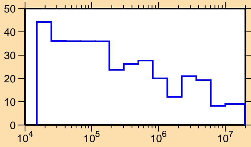
\Delta\sigma/\sigma vs. E for ^{183}\text{Ir}(n,\text{tot.})
