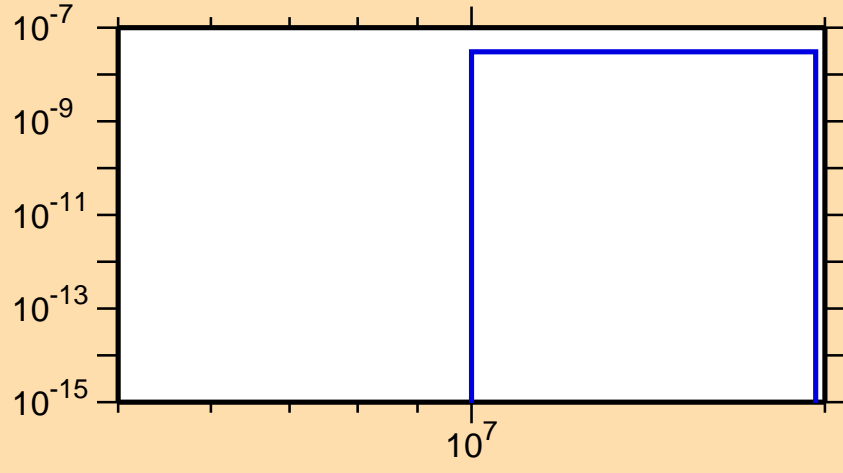
\sigma vs. E for ^{183}\text{Ir}(n,\text{He3})
