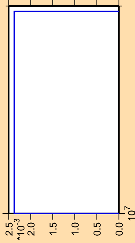
\Delta\sigma/\sigma vs. E for ^{183}\text{Ir}(n,3n\alpha)
