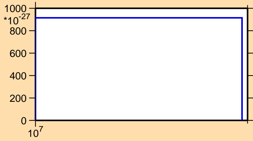
\sigma vs. E for ^{183}\text{Ir} (mt 42)
