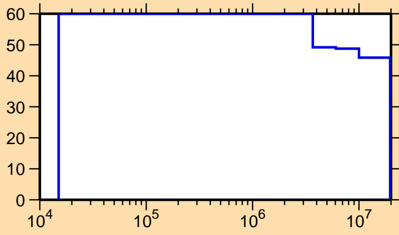
\Delta\sigma/\sigma vs. E for ^{183}\text{Ir}(n,n_1)
