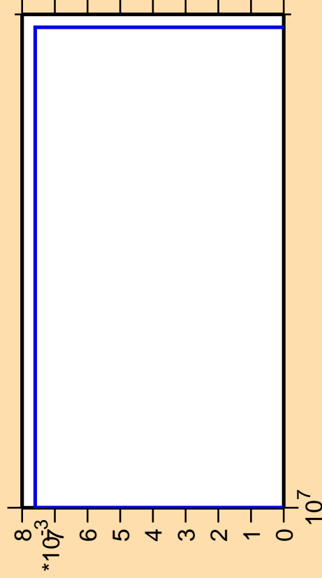
\Delta\sigma/\sigma vs. E for ^{183}\text{Ir}(n,\text{pt})
