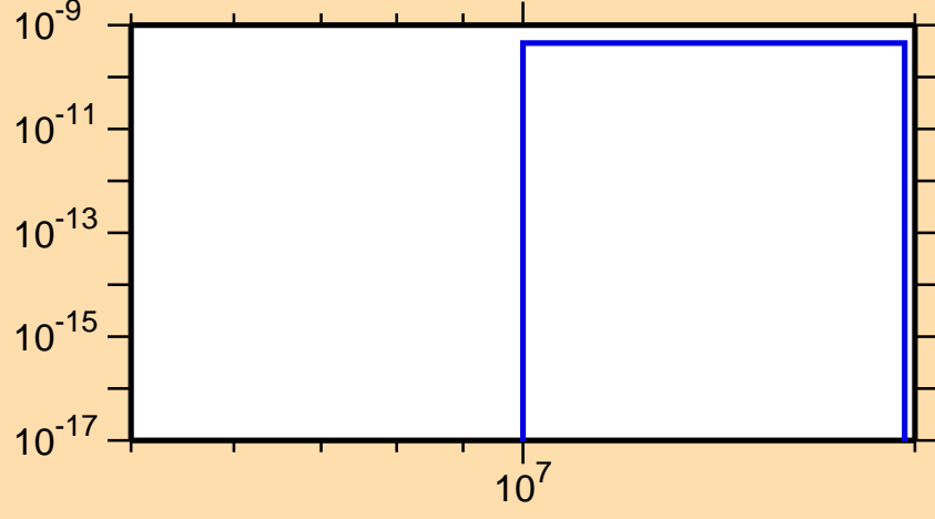
\sigma vs. E for ^{183}\text{Ir}(\text{mt } 45)
