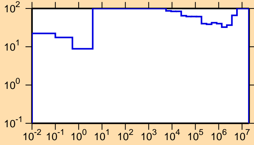
\Delta\sigma/\sigma vs. E for ^{183}\text{Ir}(n,\gamma)
