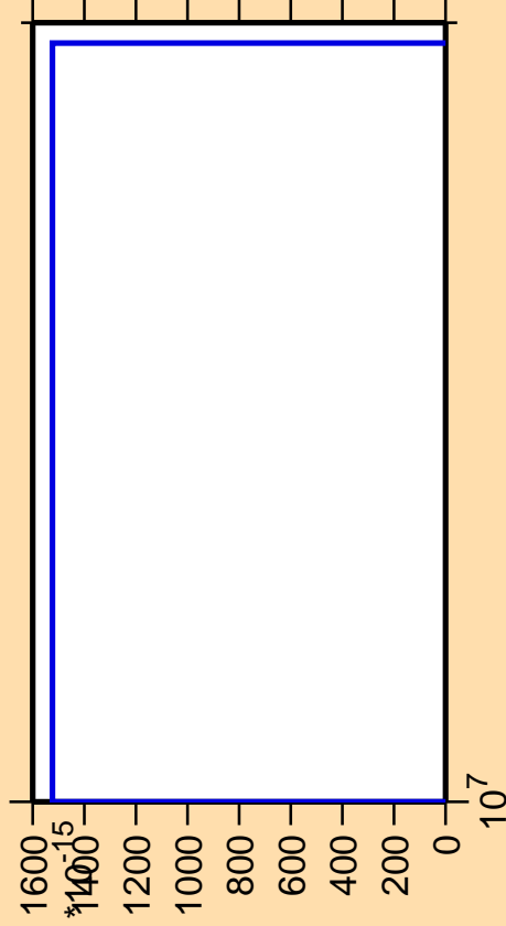
\Delta\sigma/\sigma vs. E for ^{183}\text{Ir} (mt 42)
