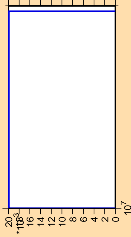
\Delta\sigma/\sigma vs. E for ^{183}\text{Ir} (mt 34)
