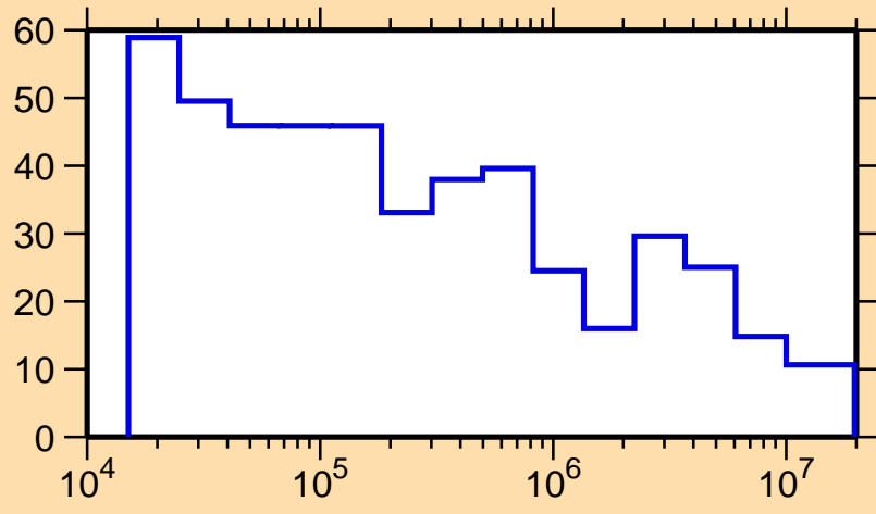
\Delta\sigma/\sigma vs. E for ^{183}\text{Ir}(n,\text{el.})
