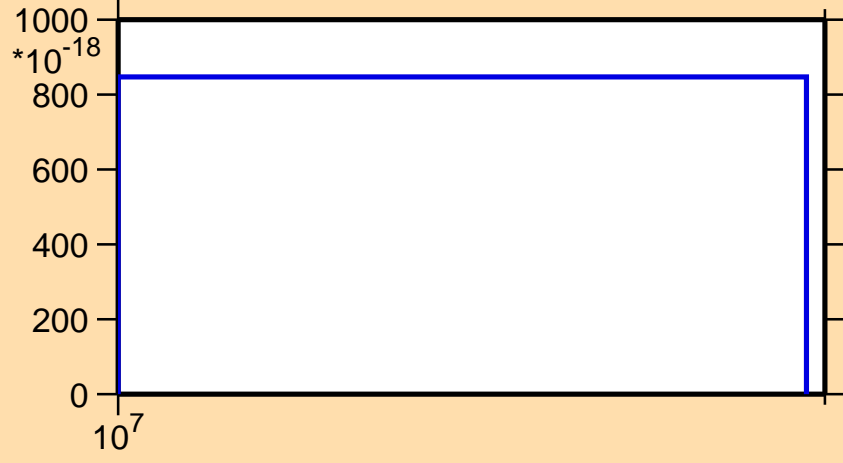
\sigma vs. E for ^{183}\text{Ir}(n,\text{pt})
