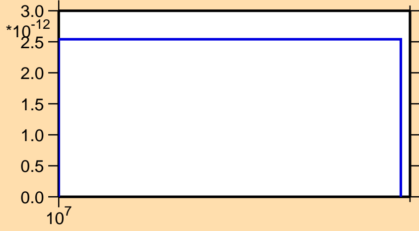
\sigma vs. E for ^{183}\text{Ir}(n,\text{pd})
