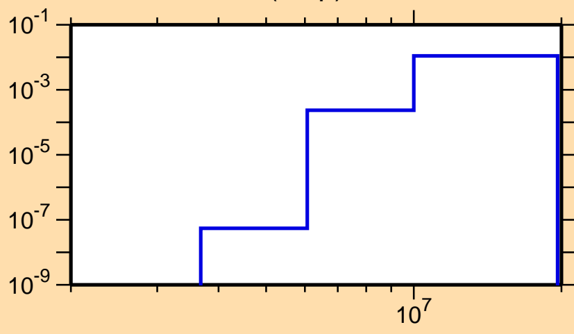
\sigma vs. E for ^{183}\text{Ir}(n,np)
