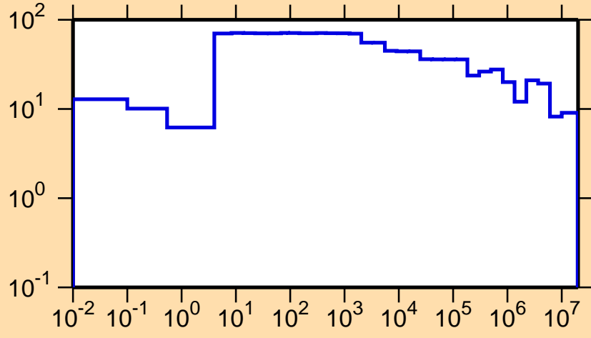
\Delta\sigma/\sigma vs. E for ^{183}\text{Ir}(n,\text{tot.})
