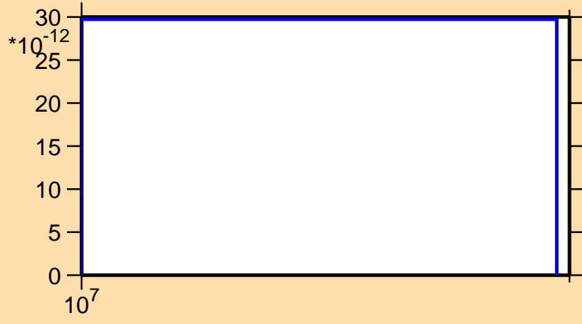
\sigma vs. E for ^{183}\text{Ir}(\text{mt117})
