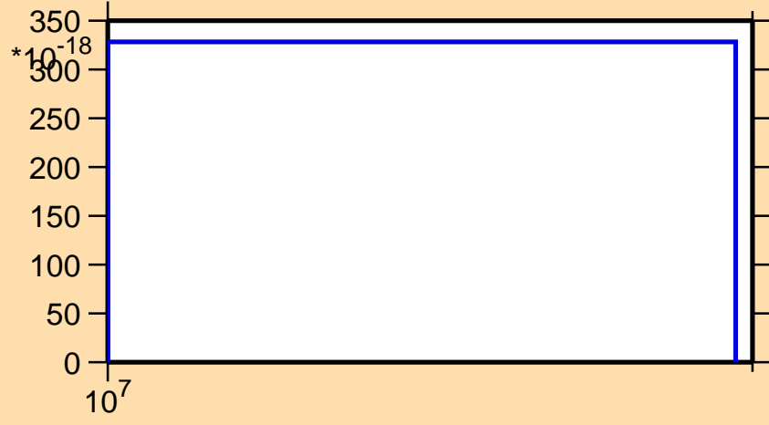
\sigma vs. E for ^{183}\text{Ir}(n,3n\alpha)
