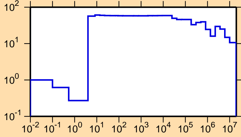
\Delta\sigma/\sigma vs. E for ^{183}\text{Ir}(n,\text{el.})
