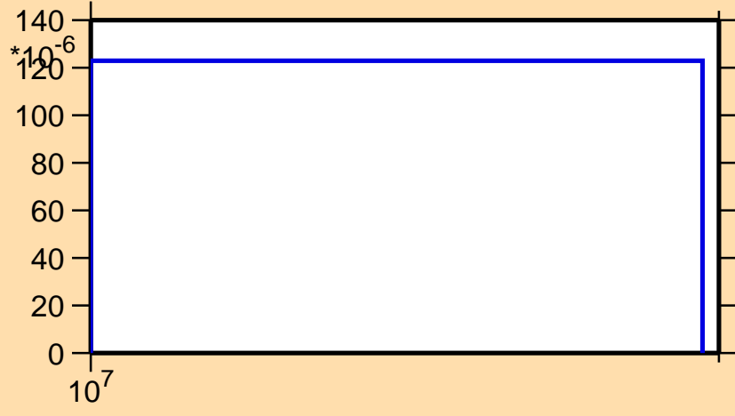
\sigma vs. E for ^{183}\text{Ir}(n,3n)
