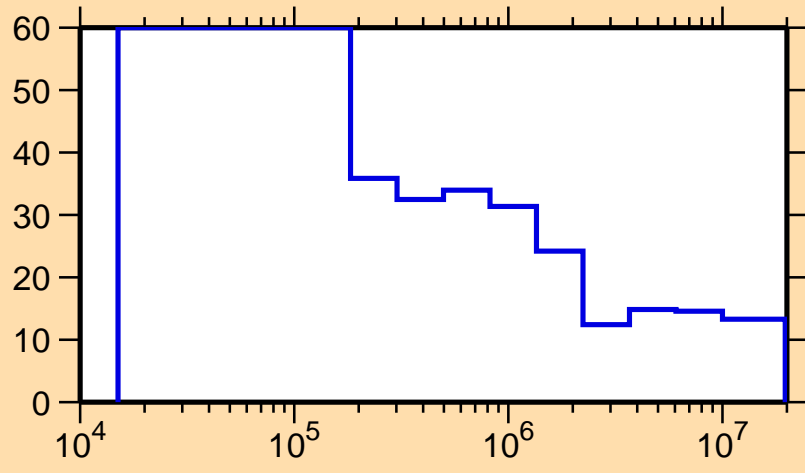
\Delta\sigma/\sigma vs. E for ^{183}\text{Ir}(n,\text{nonel.})
