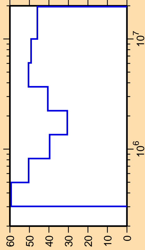
\Delta\sigma/\sigma vs. E for ^{183}\text{Ir}(n,n_4)
