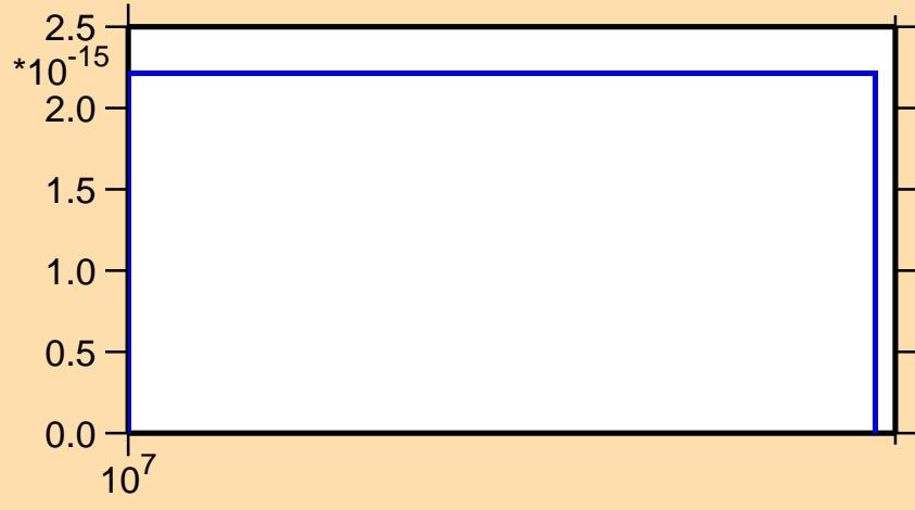
\sigma vs. E for ^{183}\text{Ir} (mt 34)
