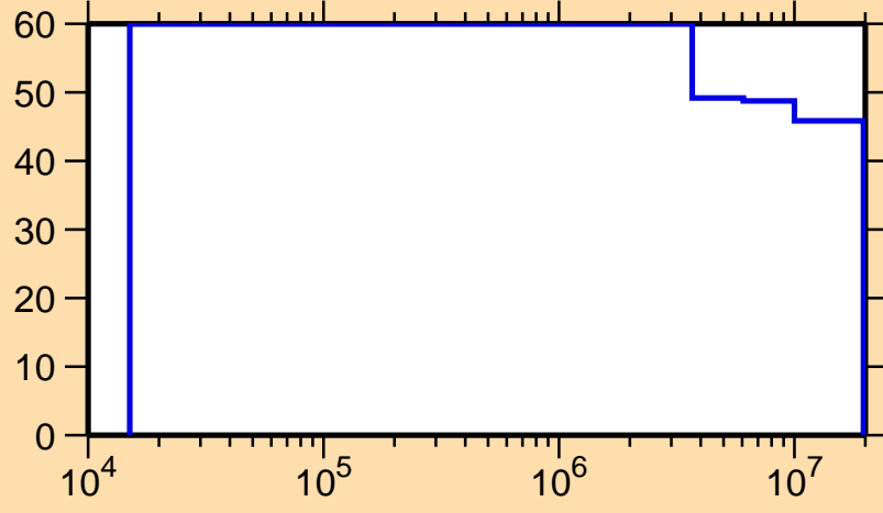
\Delta\sigma/\sigma vs. E for ^{183}\text{Ir}(n,n_1)
