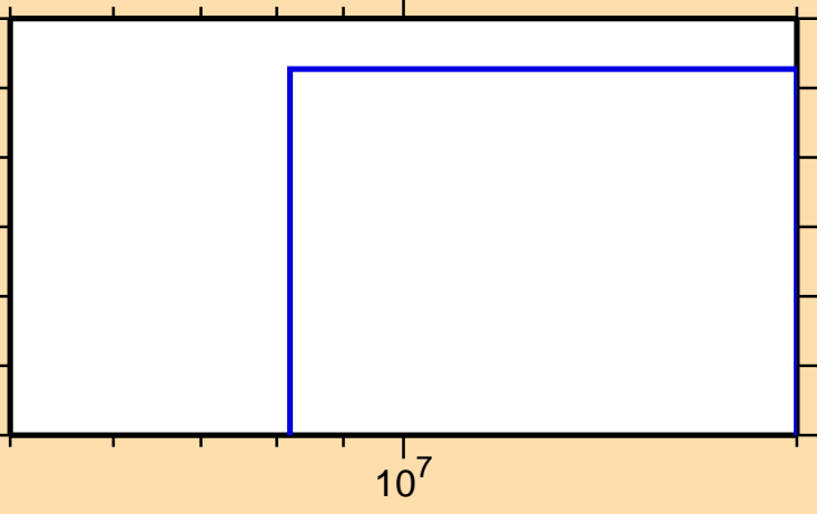
\sigma vs. E for ^{183}\text{Ir}(n,3n)
