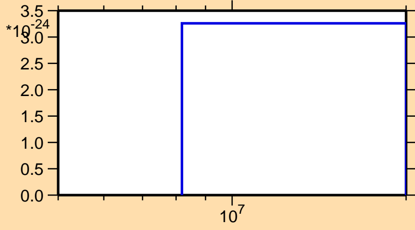
\sigma vs. E for ^{183}\text{Ir}(\text{mt } 42)
