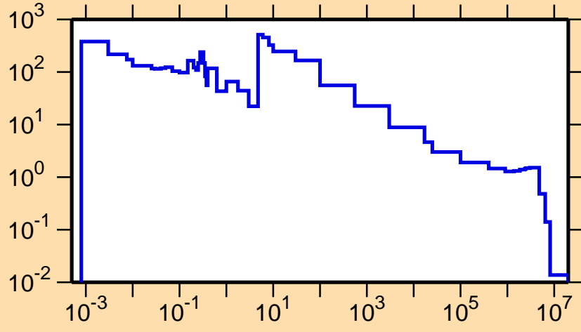
\sigma vs. E for ^{183}\text{Ir}(n,\gamma)
