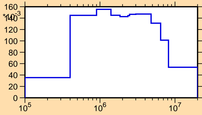
\sigma vs. E for ^{183}\text{Ir}(n,n_2)
