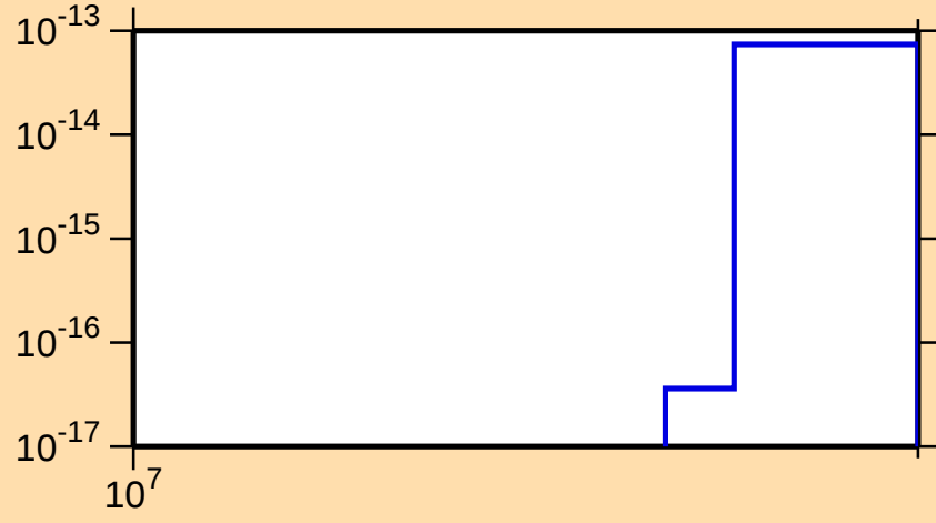
\sigma vs. E for ^{185}\text{Ir}(\text{mt } 34)
