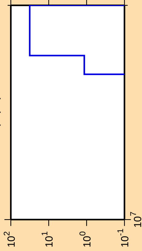
\Delta\sigma/\sigma vs. E for ^{185}\text{Ir}(n,\text{pd})
