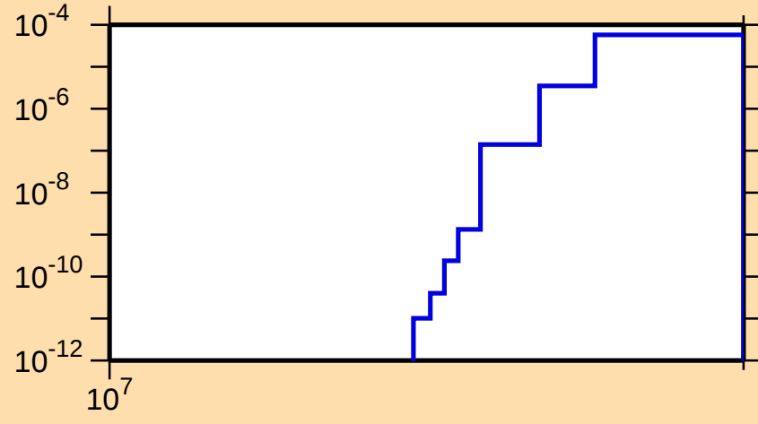
\sigma vs. E for ^{185}\text{Ir}(n,2np)
