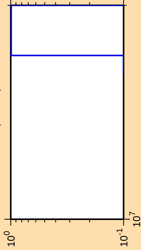
\Delta\sigma/\sigma vs. E for ^{185}\text{Ir}(n,3n\alpha)
