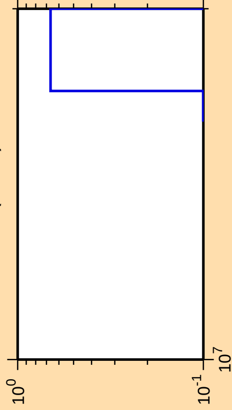
\Delta\sigma/\sigma vs. E for ^{185}\text{Ir}(\text{mt } 34)
