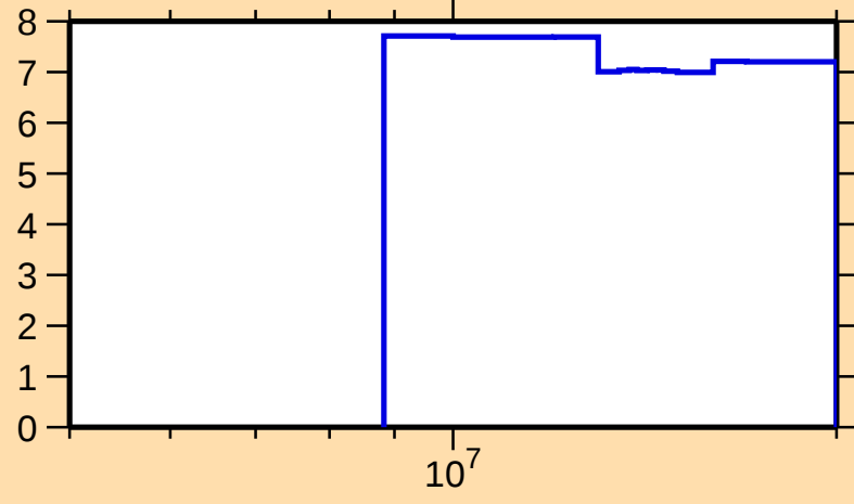
\Delta\sigma/\sigma vs. E for ^{185}\text{Ir}(n,\text{nonel.})
