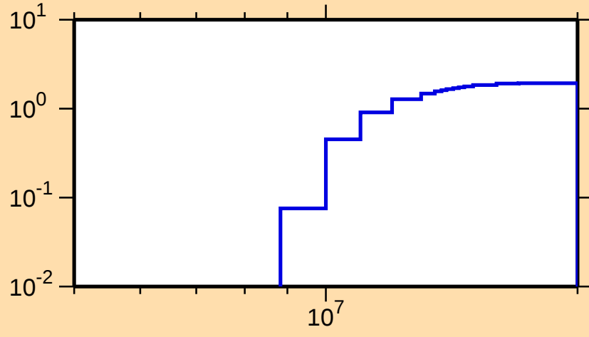
\sigma vs. E for ^{185}\text{Ir}(n,2n)
