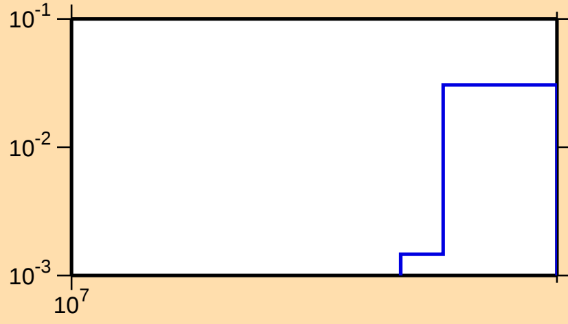
\sigma vs. E for ^{185}\text{Ir}(n,3n)
