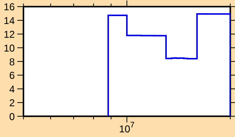
\Delta\sigma/\sigma vs. E for ^{185}\text{Ir}(n,\text{el.})
