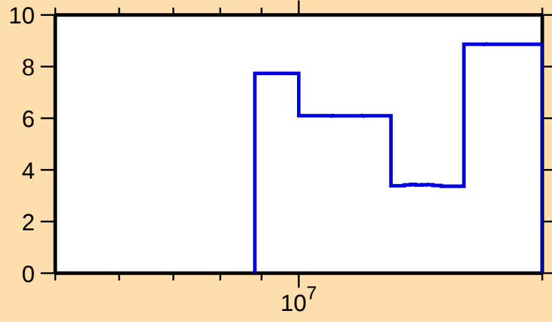
\Delta\sigma/\sigma vs. E for ^{185}\text{Ir}(n,\text{tot.})
