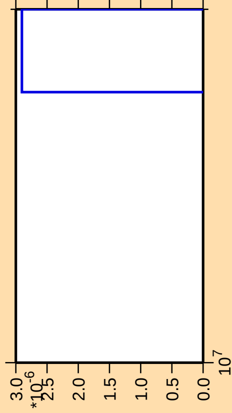
\Delta\sigma/\sigma vs. E for ^{185}\text{Ir}(\text{mt } 42)
