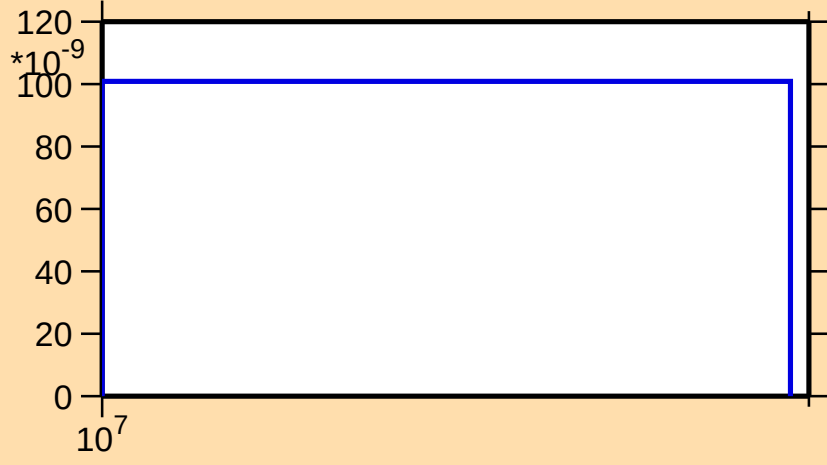
\sigma vs. E for ^{185}\text{Ir}(n,\text{nd})
