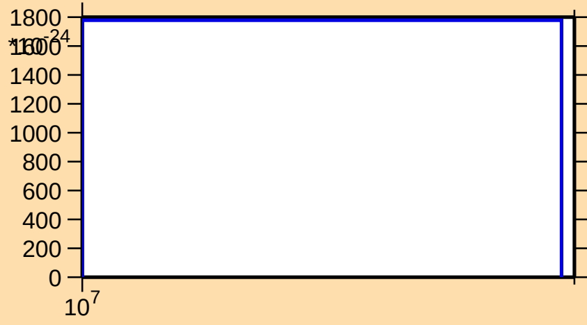
\sigma vs. E for ^{185}\text{Ir}(\text{mt } 42)
