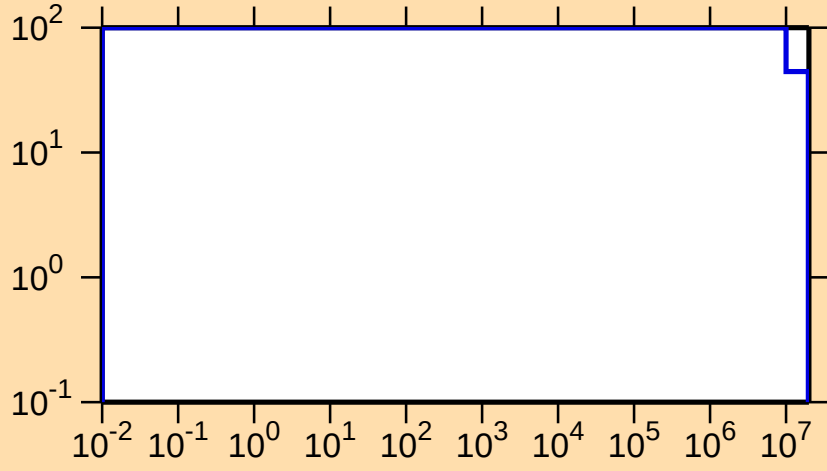
\Delta\sigma/\sigma vs. E for ^{185}\text{Ir}(n,p)
