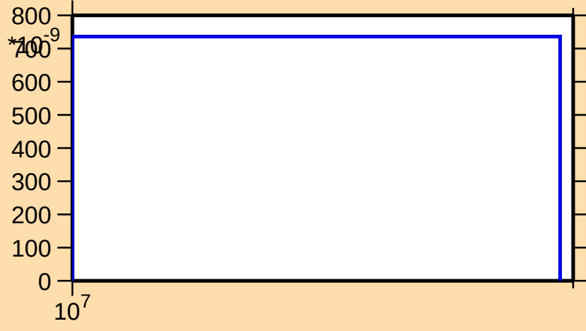
\sigma vs. E for ^{185}\text{Ir}(n,2np)
