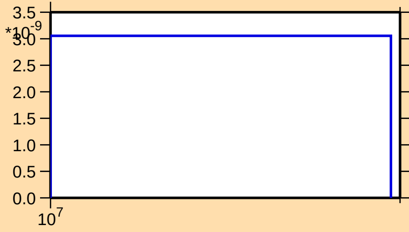
\sigma vs. E for ^{185}\text{Ir}(n,\text{nt})
