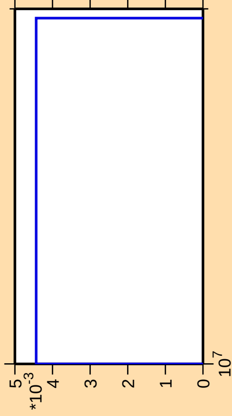
\Delta\sigma/\sigma vs. E for ^{185}\text{Ir}(\text{mt } 34)
