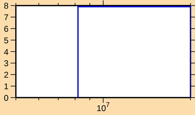
\Delta\sigma/\sigma vs. E for ^{185}\text{Ir}(n,\text{el.})
