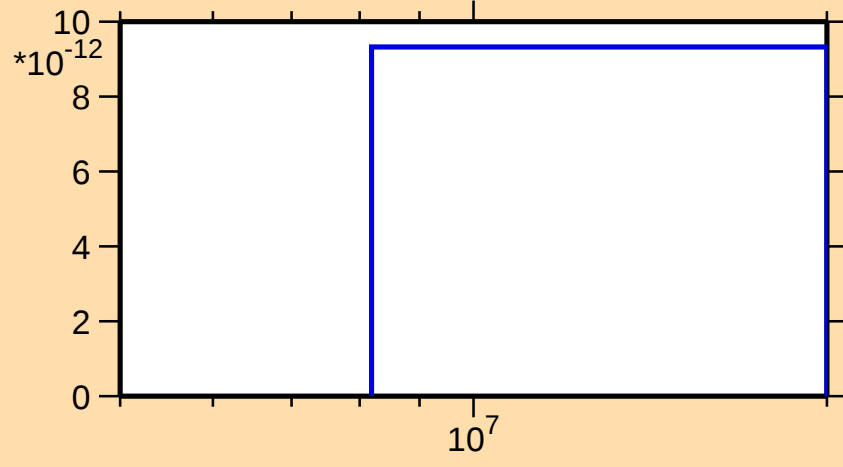
\sigma vs. E for ^{185}\text{Ir}(\text{mt } 45)
