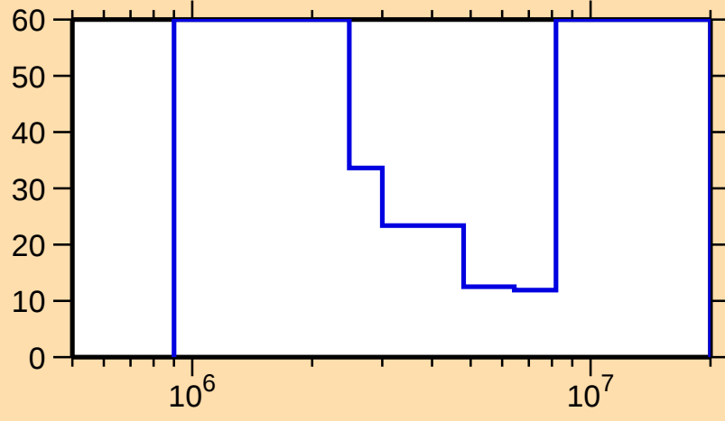
\Delta\sigma/\sigma vs. E for ^{185}\text{Ir}(\text{n},\text{inel.})
