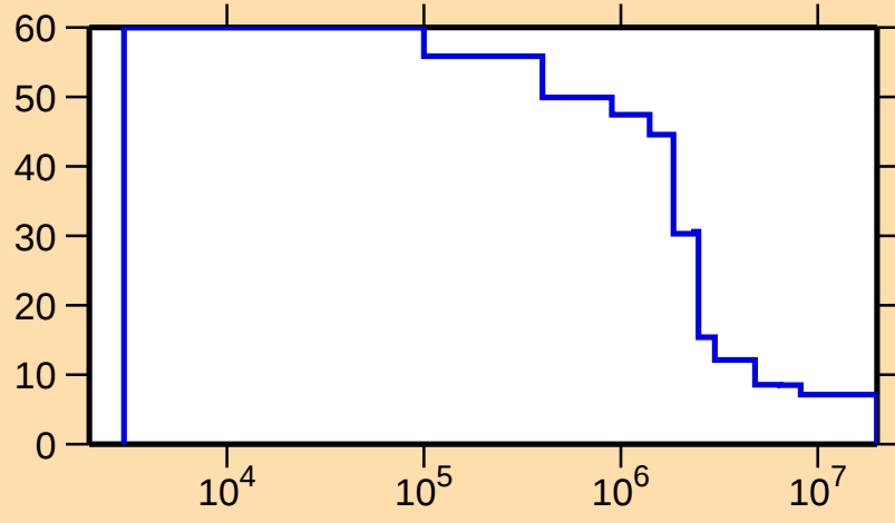
\Delta\sigma/\sigma vs. E for ^{185}\text{Ir}(n,\text{nonel.})
