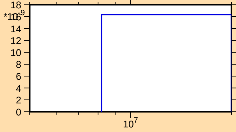
\sigma vs. E for ^{185}\text{Ir}(n,2n\alpha)
