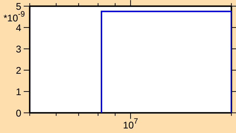
\sigma vs. E for ^{185}\text{Ir}(n,\text{He3})
