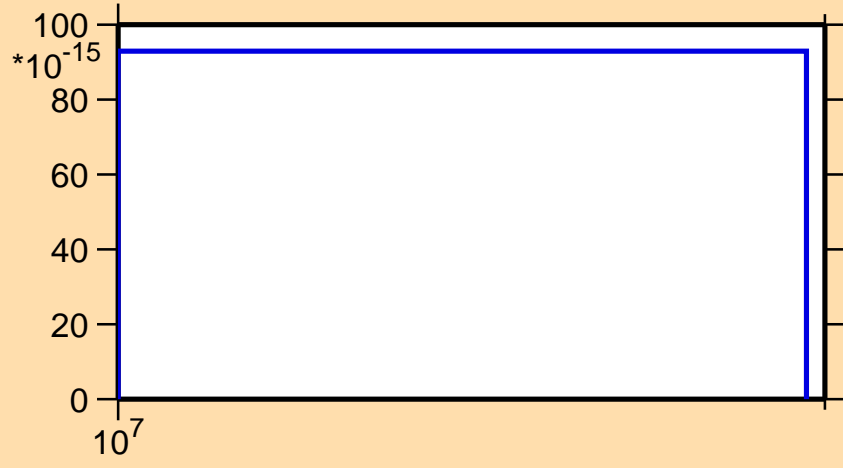
\sigma vs. E for ^{186}\text{Ir} (mt 34)
