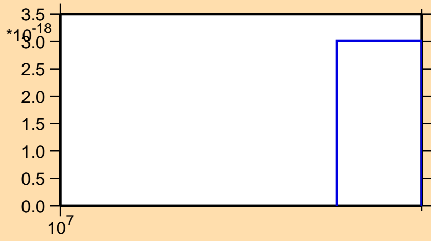
\sigma vs. E for ^{188}\text{Ir}(\text{mt } 42)
