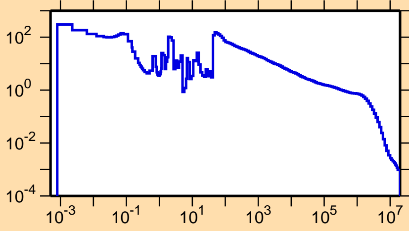
\sigma vs. E for ^{188}\text{Ir}(n,\gamma)
