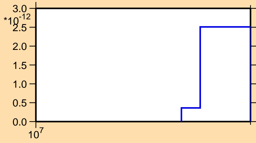
\sigma vs. E for ^{188}\text{Ir}(\text{mt117})
