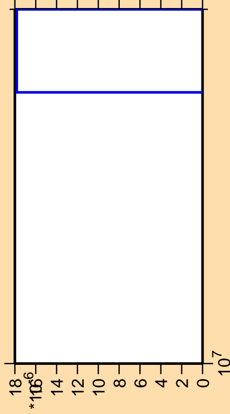
\Delta\sigma/\sigma vs. E for ^{188}\text{Ir}(\text{mt } 42)
