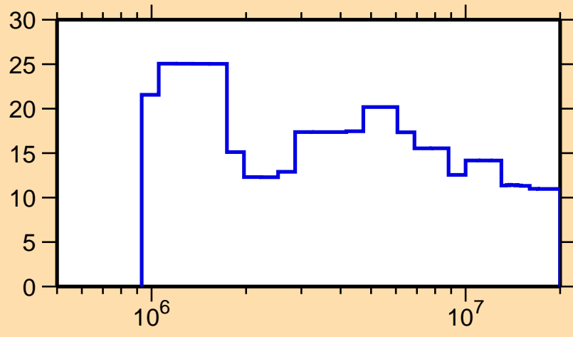
\Delta\sigma/\sigma vs. E for ^{188}\text{Ir}(n,el.)
