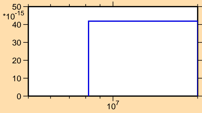
\sigma vs. E for ^{188}\text{Ir}(\text{mt } 45)
