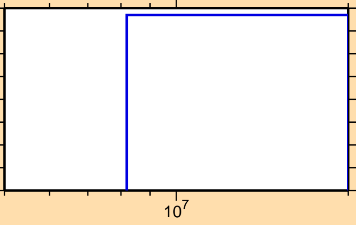
\sigma vs. E for ^{188}\text{Ir}(n,3n\alpha)
