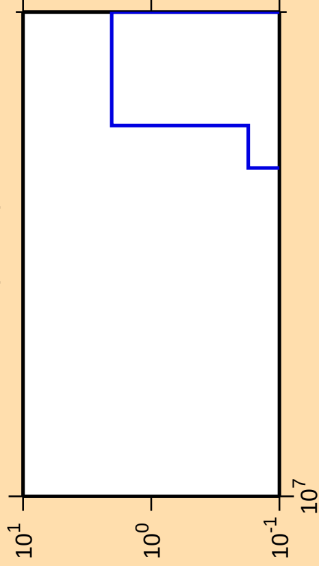
\Delta\sigma/\sigma vs. E for ^{189}\text{Ir} (mt 45)
