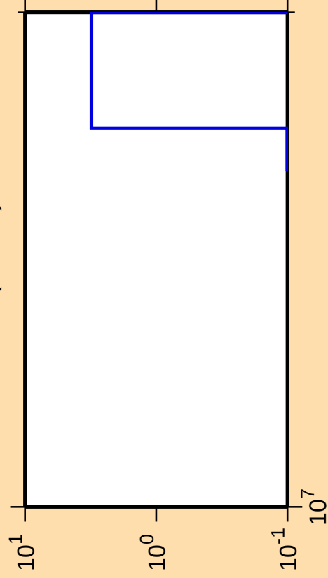
\Delta\sigma/\sigma vs. E for ^{189}\text{Ir}(n,3n\alpha)
