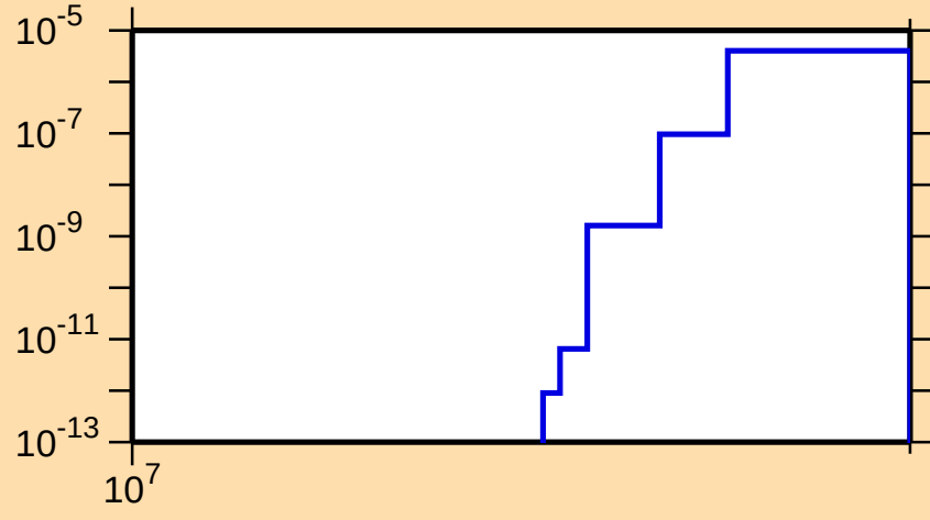
\sigma vs. E for ^{189}\text{Ir}(n,2np)
