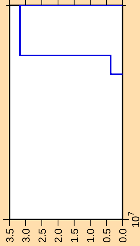
\Delta\sigma/\sigma vs. E for ^{189}\text{Ir}(\text{mt117})
