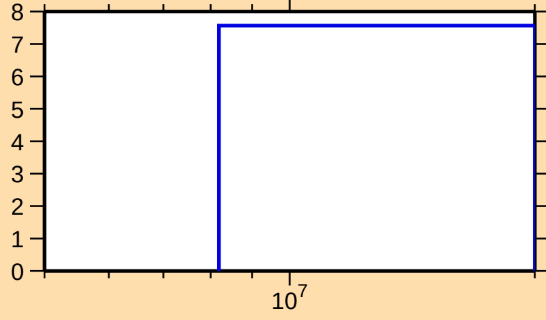
\Delta\sigma/\sigma vs. E for ^{189}\text{Ir}(n,\text{el.})
