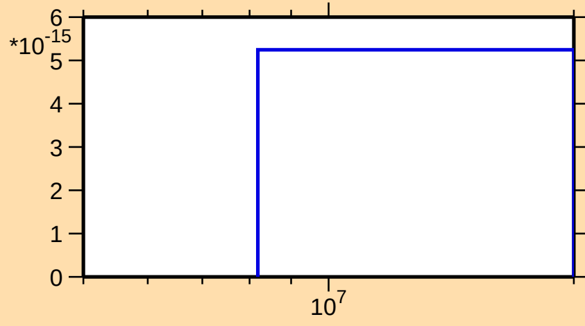
\sigma vs. E for ^{189}\text{Ir}(\text{mt } 45)
