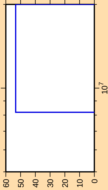
\Delta\sigma/\sigma vs. E for ^{189}\text{Ir}(n,p)
