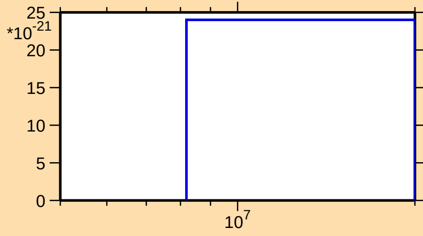
\sigma vs. E for ^{189}\text{Ir}(\text{mt } 42)
