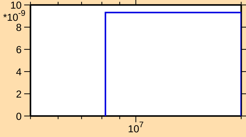
\sigma vs. E for ^{189}\text{Ir}(n,\text{nt})
