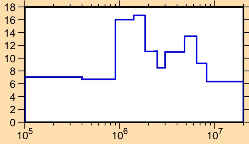
\Delta\sigma/\sigma vs. E for ^{190}\text{Ir}(n, el.)
