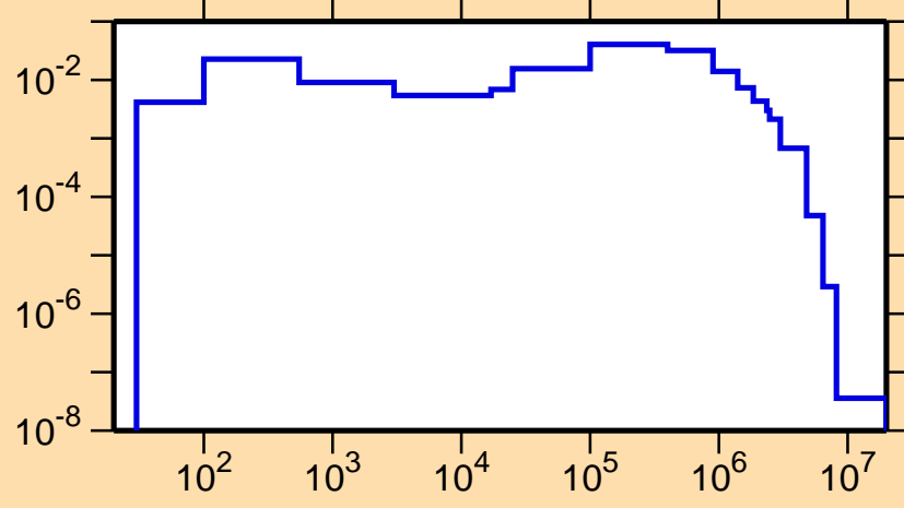
\sigma vs. E for ^{190}\text{Ir}(n,n_1)
