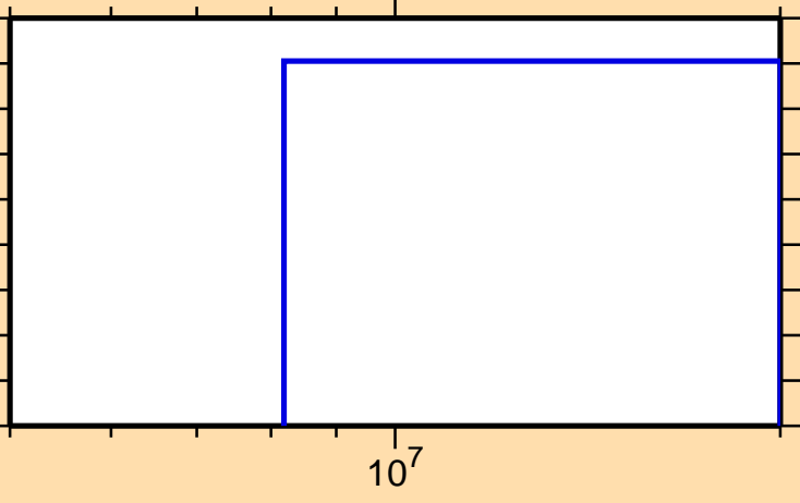
\sigma vs. E for ^{190}\text{Ir}(n,3n\alpha)
