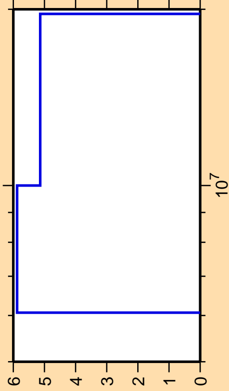
\Delta\sigma/\sigma vs. E for ^{191}\text{Ir}(n,2n)
