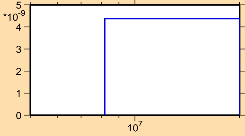
\sigma vs. E for ^{191}\text{Ir}(n,2np)
