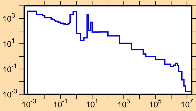
\sigma vs. E for ^{191}\text{Ir}(n,\gamma)
