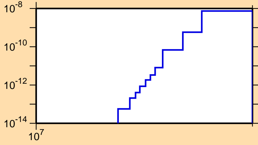
\sigma vs. E for ^{191}\text{Ir}(n,\text{He}3)
