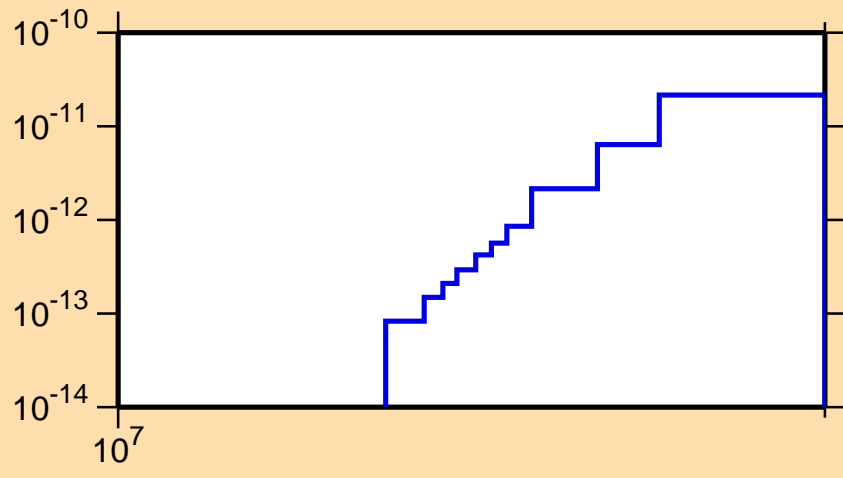
\sigma vs. E for ^{191}\text{Ir}(n,p\alpha)
