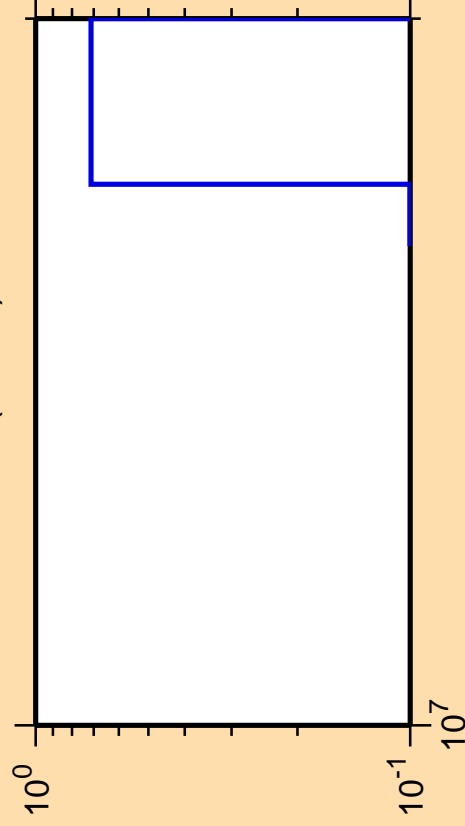
\Delta\sigma/\sigma vs. E for ^{191}\text{Ir} (mt 42)
