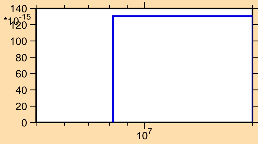
\sigma vs. E for ^{191}\text{Ir}(\text{mt } 11)
