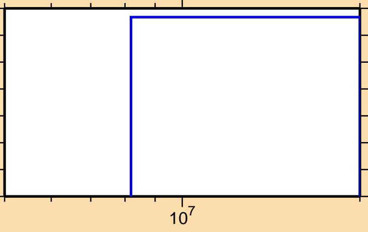
\sigma vs. E for ^{191}\text{Ir}(\text{mt } 42)
