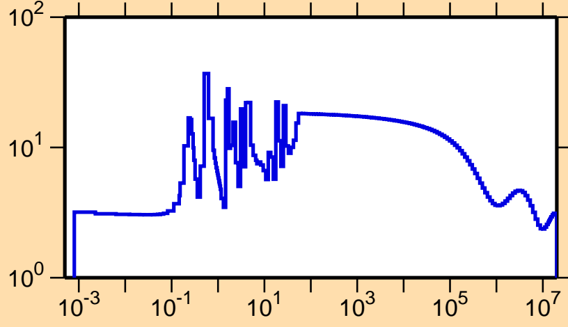
\sigma vs. E for ^{192}\text{Ir}(n,\text{el.})
