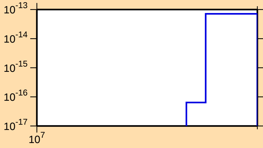
\sigma vs. E for ^{192}\text{Ir}(n,3n\alpha)
