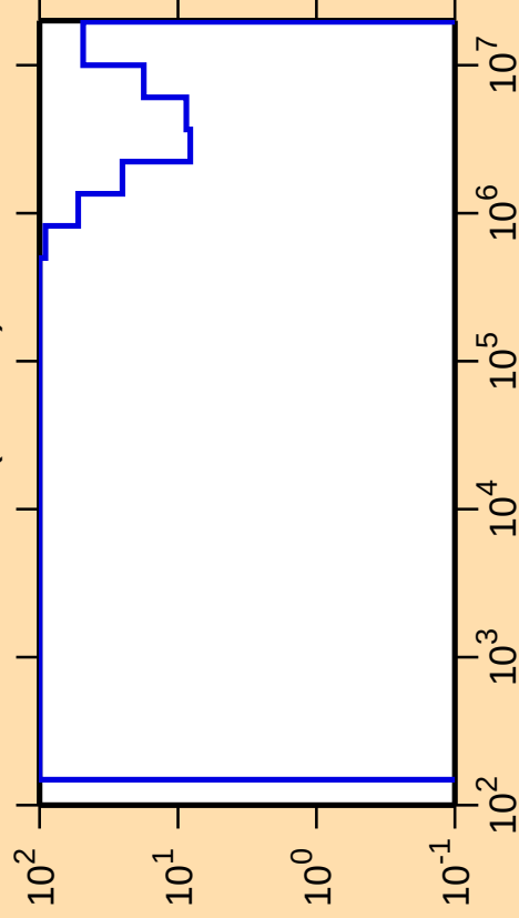
\Delta\sigma/\sigma vs. E for ^{192}\text{Ir}(n,\text{inel.})
