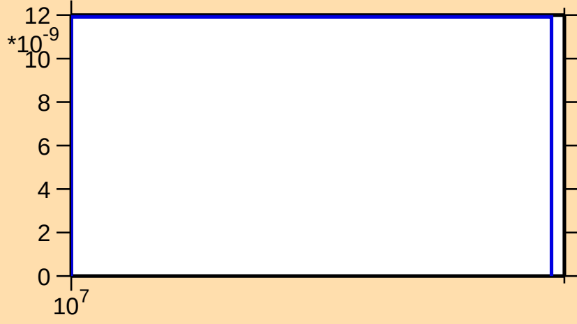
\sigma vs. E for ^{192}\text{Ir}(n,\text{nt})
