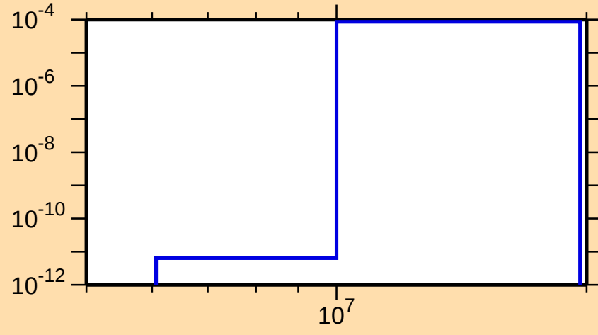
\sigma vs. E for ^{192}\text{Ir}(n,t)
