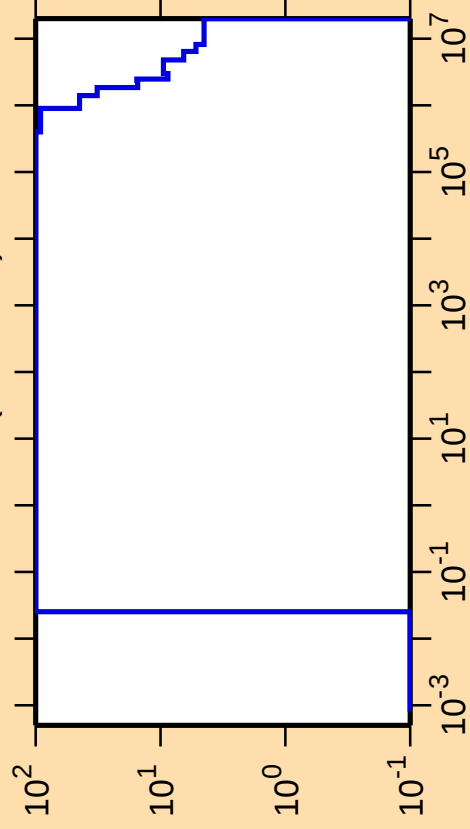
\Delta\sigma/\sigma vs. E for ^{192}\text{Ir}(n,\text{nonel.})
