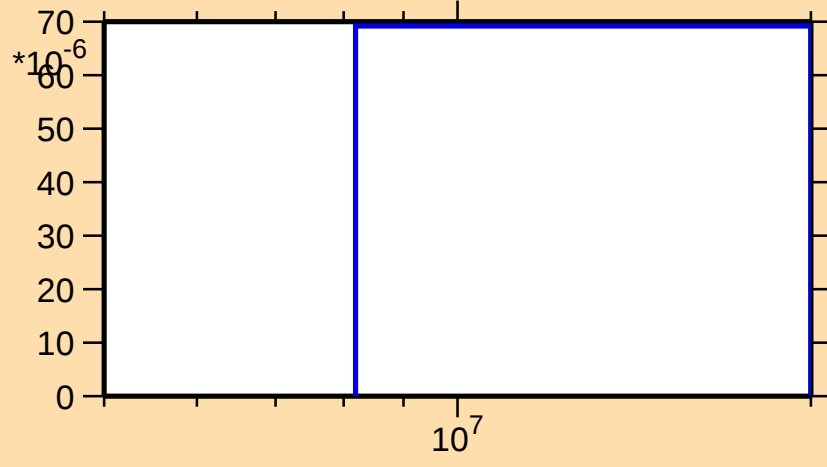
\sigma vs. E for ^{192}\text{Ir}(n,t)
