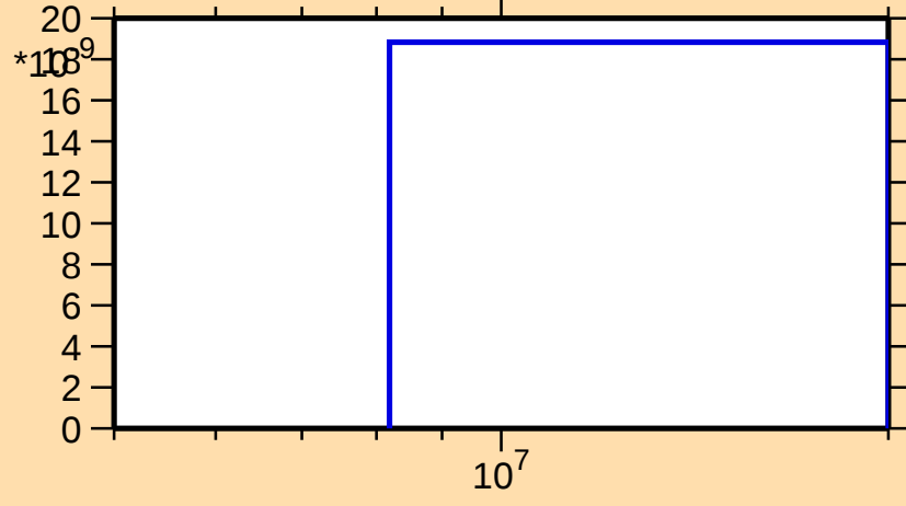
\sigma vs. E for ^{192}\text{Ir}(n,2n\alpha)
