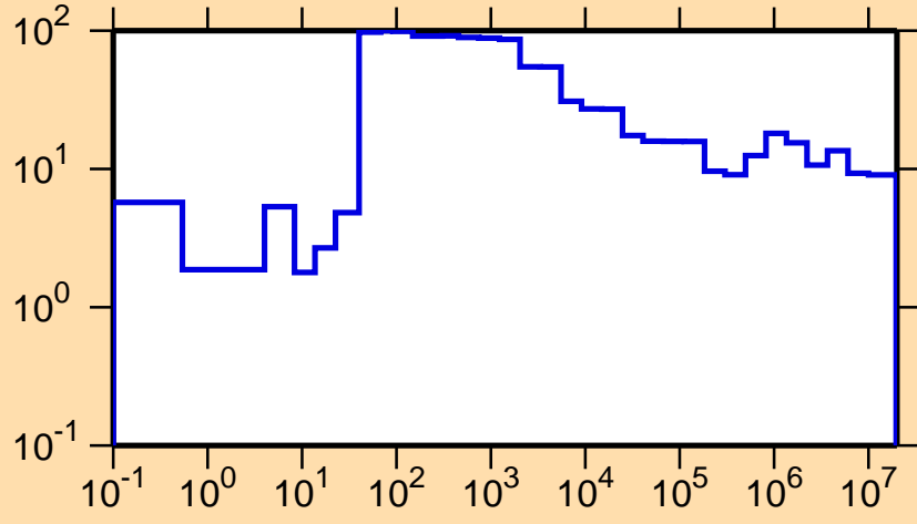
\Delta\sigma/\sigma vs. E for ^{192}\text{Ir}(n, el.)
