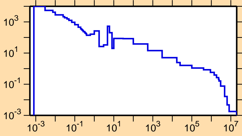
\sigma vs. E for ^{192}\text{Ir}(n,\gamma)
