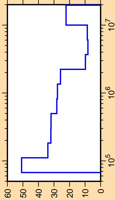
\Delta\sigma/\sigma vs. E for ^{193}\text{Ir}(n,\text{inel.})
