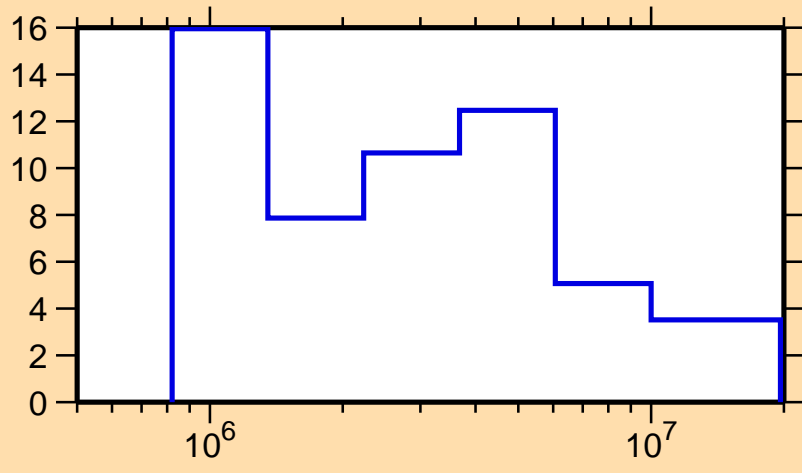
\Delta\sigma/\sigma vs. E for ^{193}\text{Ir}(n,\text{tot.})
