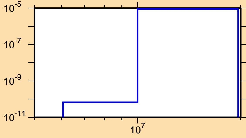
\sigma vs. E for ^{193}\text{Ir}(n,\alpha)
