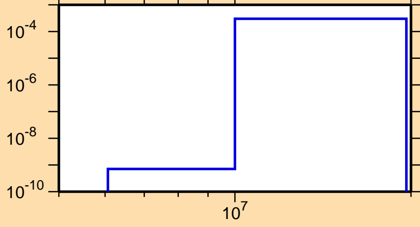
\sigma vs. E for ^{193}\text{Ir}(n,d)
