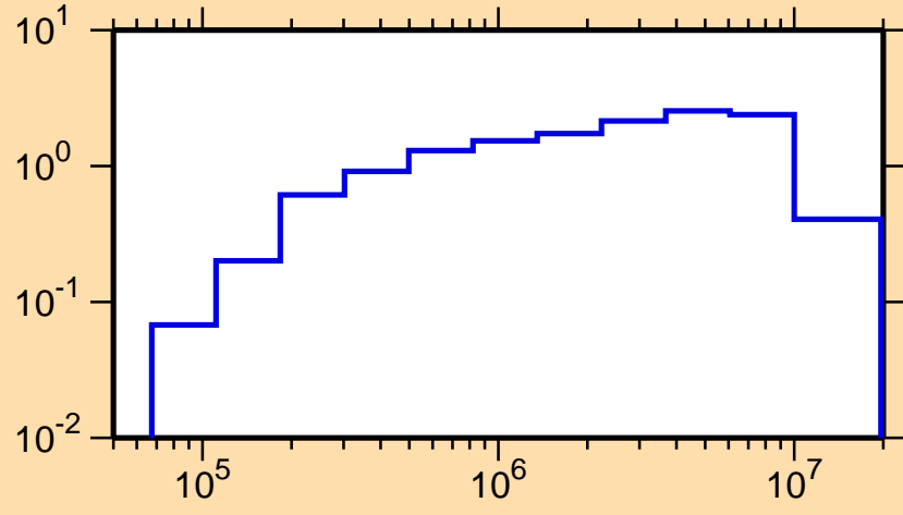
\sigma vs. E for ^{193}\text{Ir}(n,\text{inel.})
