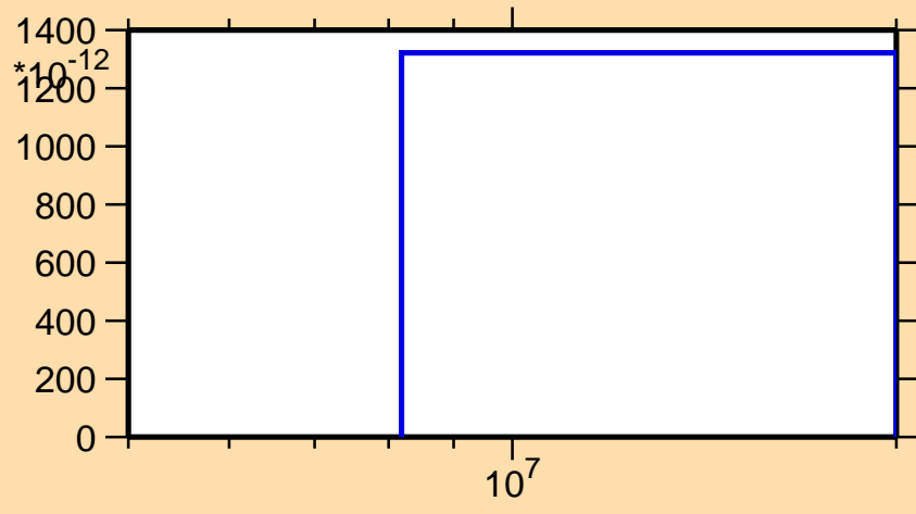
\sigma vs. E for ^{193}\text{Ir}(n,2np)
