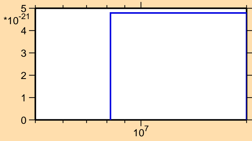
\sigma vs. E for ^{193}\text{Ir}(\text{mt } 42)
