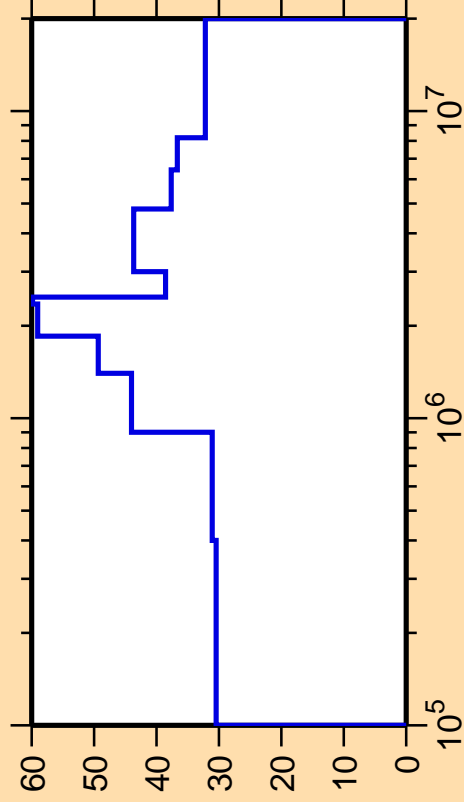
\Delta\sigma/\sigma vs. E for ^{193}\text{Ir}(n,n_4)
