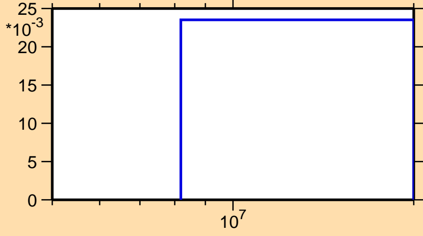
\sigma vs. E for ^{193}\text{Ir}(n,3n)
