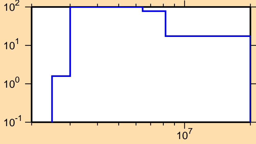
\Delta\sigma/\sigma vs. E for ^{193}\text{Ir}(n,p)
