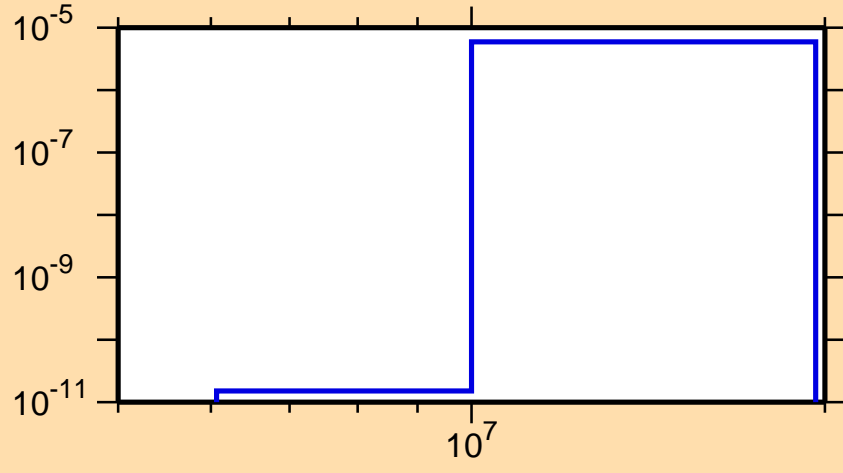
\sigma vs. E for ^{194}\text{Ir}(n,\alpha)
