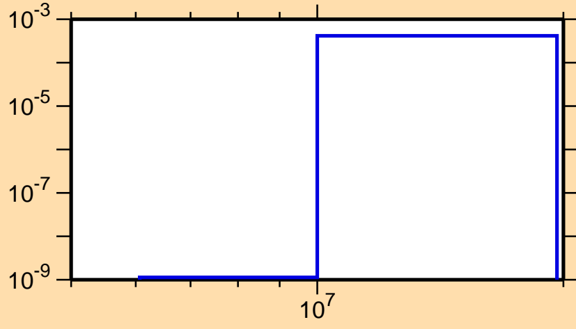
\sigma vs. E for ^{194}\text{Ir}(n,d)
